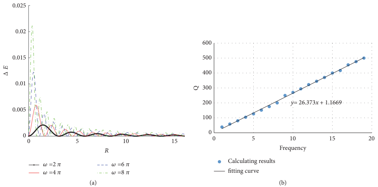
FIGURE 12: \Delta E and Q under different frequencies. (a) \Delta E at Z = 0 ; (b) Q .
