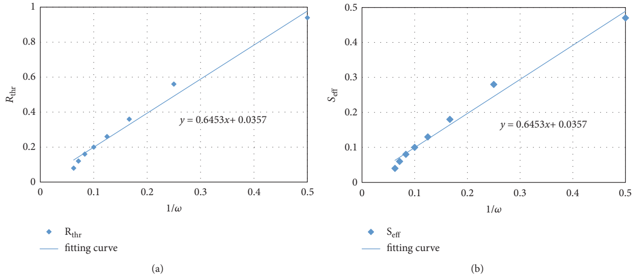
FIGURE 11: Relationship between R_{thr} s and S_{eff} s on one side and 1/\omega s on the other. Diamonds represent calculating results and blue lines represent the fitting curve.
