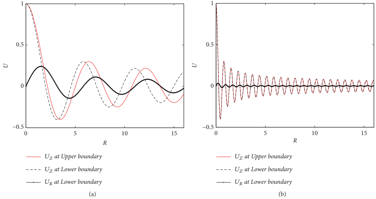
FIGURE 3: Amplitudes of tissue displacements at the upper ( Z = -L_0/u_0 ) and lower ( Z = 0 ) boundaries. (a) \omega = 2\pi ; (b) \omega = 16\pi .
