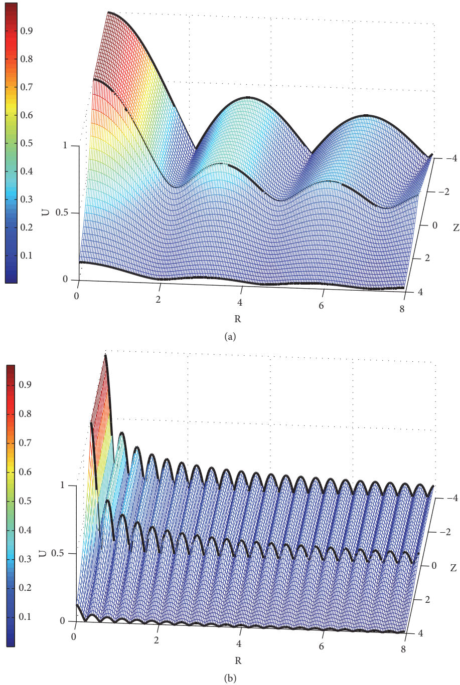
FIGURE 8: Amplitudes of tissue displacements; the black lines represent the displacement at Z = -L_0/u_0 = -4 , Z = 0 and Z = L_0/u_0 = 4 . (a) \omega = 2\pi ; (b) \omega = 16\pi .
