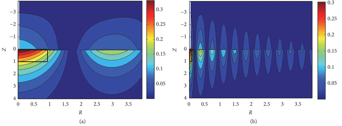
FIGURE 9: Contour lines of |E_{RZ}| in the tissue; the white lines at r \rightarrow 0 \cap -4 \leq Z \leq 0 represent the needle; the black rectangles represent the approximate area where |E_{RZ}| > 0.2 . (a) \omega = 2\pi ; (b) \omega = 16\pi .
