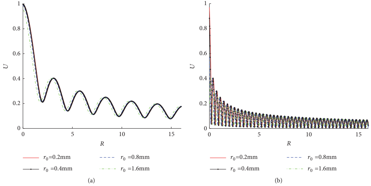
FIGURE 7: Amplitudes of tissue displacements under different r_0 s. (a) \omega = 2\pi ; (b) \omega = 16\pi .
