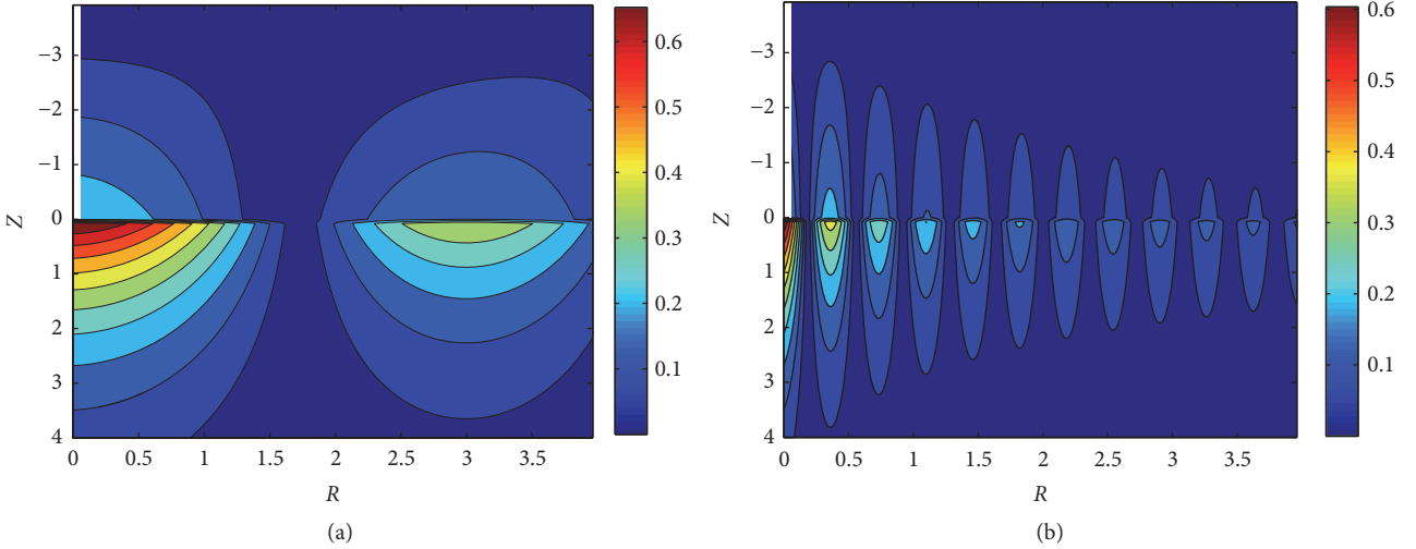
FIGURE 10: Contour lines of |T_{RZ}| in the tissue, the white lines at R \rightarrow 0 \cap -4 \leq Z \leq 0 represent the needle. (a) \omega = 2\pi ; (b) \omega = 16\pi .
