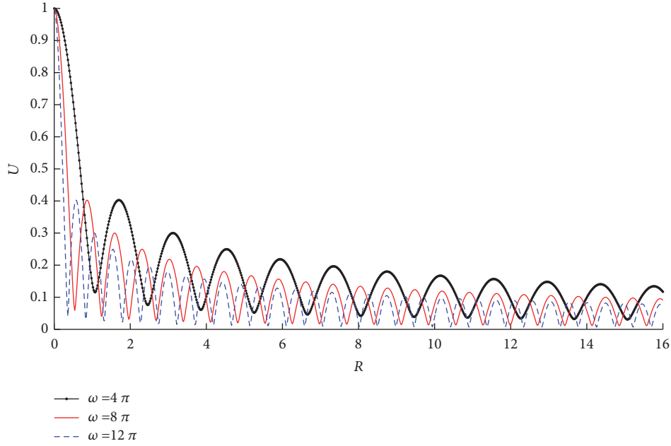
FIGURE 5: Amplitudes of tissue displacements under different frequencies.
