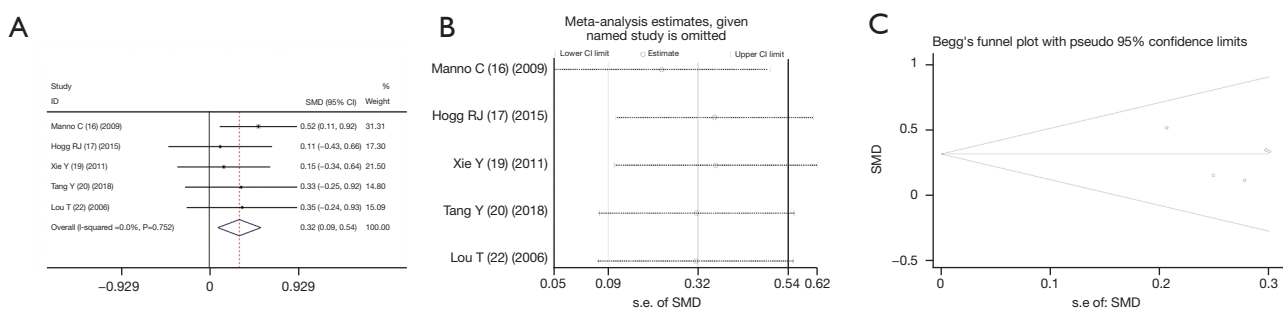
Figure 6 Forest plot, sensitivity analysis, and funnel plot of meta-analysis of glomerular filtration rate. SMD, standardized mean difference.
