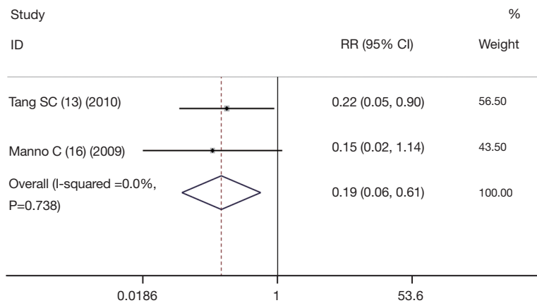
Figure 4 Forest plot of meta-analysis of end-stage kidney disease. RR, relative risk.
