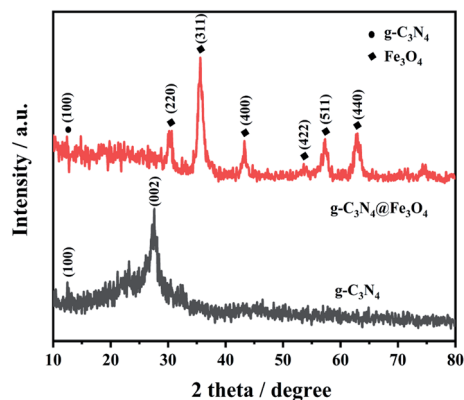
Fig. 3 XRD patterns of g\text{-C}_3\text{N}_4 and g\text{-C}_3\text{N}_4@\text{Fe}_3\text{O}_4 .
