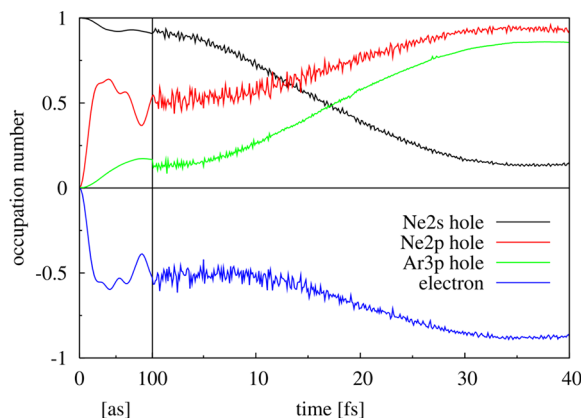
Figure 19. Hole occupation density of NeAr after Ne(2 s ) ionization in dependence of time. The initial vacancy (Ne(2 s )) is filled while the two other holes (Ne(2 p ) and Ar(3 p )) open during ICD. The blue line corresponds to the emitted ICD electron density (depicted in terms of an electron hole). Reprinted with permission from ref 227. Copyright 2007 APS.
