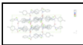
Fig. 2. Part of the crystal structure of the title compound. Molecular chains are generated by N—H···O hydrogen bonds which are shown by dashed lines. H atoms not involved in intermolecular bonding have been omitted.
