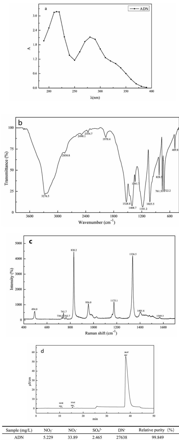
Fig. 16 UV-visible spectrum (a), IR spectrum (b), Raman spectrum (c) and ion chromatogram (d) of the purified ADN.
