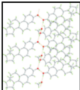
Fig. 5. View of the supramolecular chain aligned along the b axis of the crystal structure of (I). The O—H...O contacts hydrogen bonds are shown as orange dashed lines. Only one orientation of the disordered O—H1 atom is shown.
