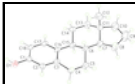
Fig. 1. The molecular structures of the first independent molecule comprising the asymmetric unit of (I) showing displacement ellipsoids at the 50% probability level.
