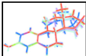
Fig. 4. Overlay diagram the three independent molecules comprising the asymmetric unit of (I) and their disordered components. The disordered components of the molecule shown in Fig. 1 are shown in red and green, the disordered components of Fig. 2 are shown in blue and pink, and the molecule in Fig. 3 is shown in light-blue.
