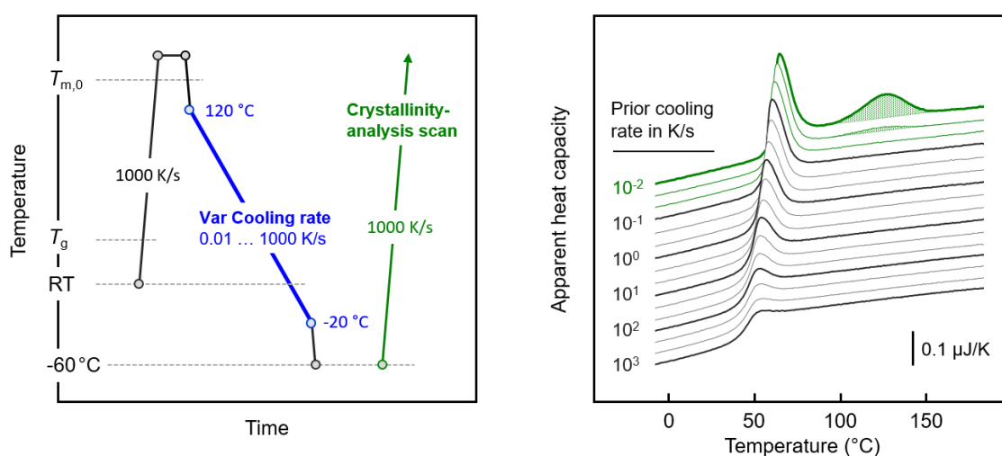
Figure 1. Temperature–time profile for the analysis of the cooling rate dependence of the crystallization of poly(butylene isophthalate) PBI (left), and fast scanning chip calorimetry (FSC) heating scans for the analysis of the formation of crystals during prior cooling at rates of 1000, 500, 200, 100, 50, 20, 10, 5, 2, 1, 0.5, 0.2, 0.1, 0.05, 0.02, and 0.01 K/s (from bottom to top) (right).
