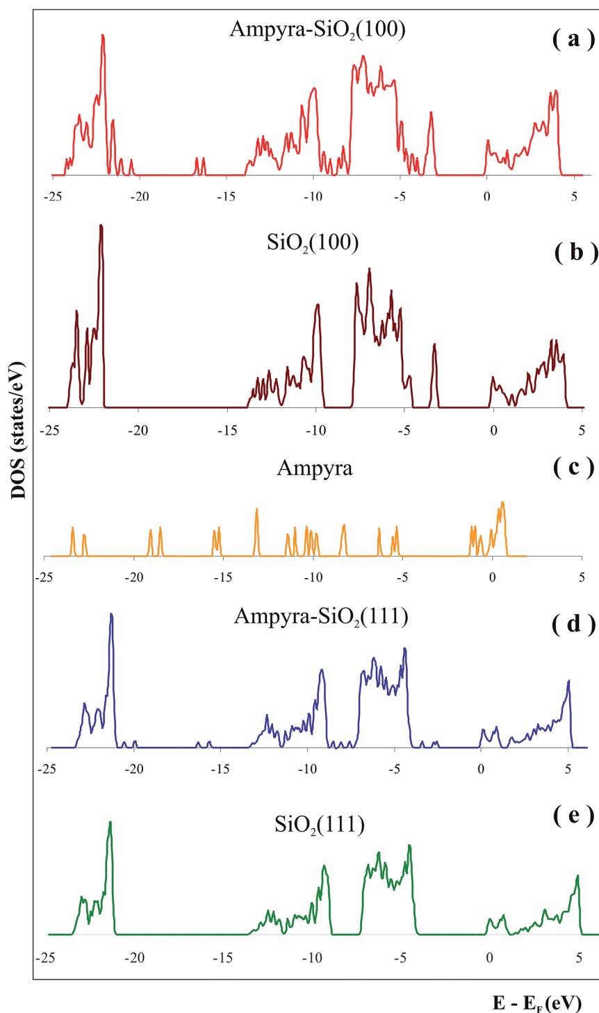
Fig. 4 Density of states (DOS) of (a) Ampyra adsorbed on SiO 2 (100) surface, (b) isolated SiO 2 (100) surface, (c) isolated Ampyra, (d) Ampyra adsorbed on SiO 2 (111) surface and (e) isolated SiO 2 (111) surface.
