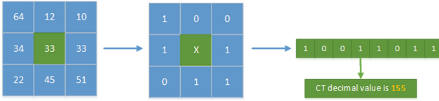
Fig. 2. Census transform
