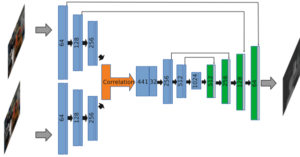
Fig. 1. FlowNet architecture.
