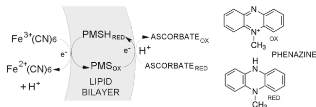
Figure 2. Establishing pH gradients in liposome preparations. Phenazine addition as phenazine methosulfate (PMS) was used as a positive control for the system. The oxidized and reduced forms of phenazine are shown on the right. Note that upon reduction a hydrogen is added to the nitrogen atom on the central ring. The hydrogen is released as a proton when the phenazine is oxidized by the ferricyanide in the liposomes, resulting in a decreased pH.
