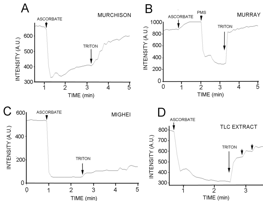
Figure 4. (A) Evidence for electron carriers in meteorite extracts. The nonpolar compounds of the Murchison meteorite organic extract were allowed to embed in liposome membranes before testing for electron carrier activity. The addition of ascorbate caused a fluorescence quenching of 56% which could be reversed with Triton X-100. The organic compounds of the Murray meteorite sample did not produce quenching when ascorbate was added (B) but addition of PMS led a quenching of fluorescence by 75% which could be reversed with Triton X-100. When the organic extract of the Mighei meteorite was added to the model system, an 86% quenching of fluorescence resulted (C) but could not be reversed with the addition of Triton X-100. The Murchison meteorite organic extract was partially purified by thin layer chromatography and one portion (see Fig. 5) also produced fluorescence quenching of 63% that was reversed by adding Triton X-100 (D).
