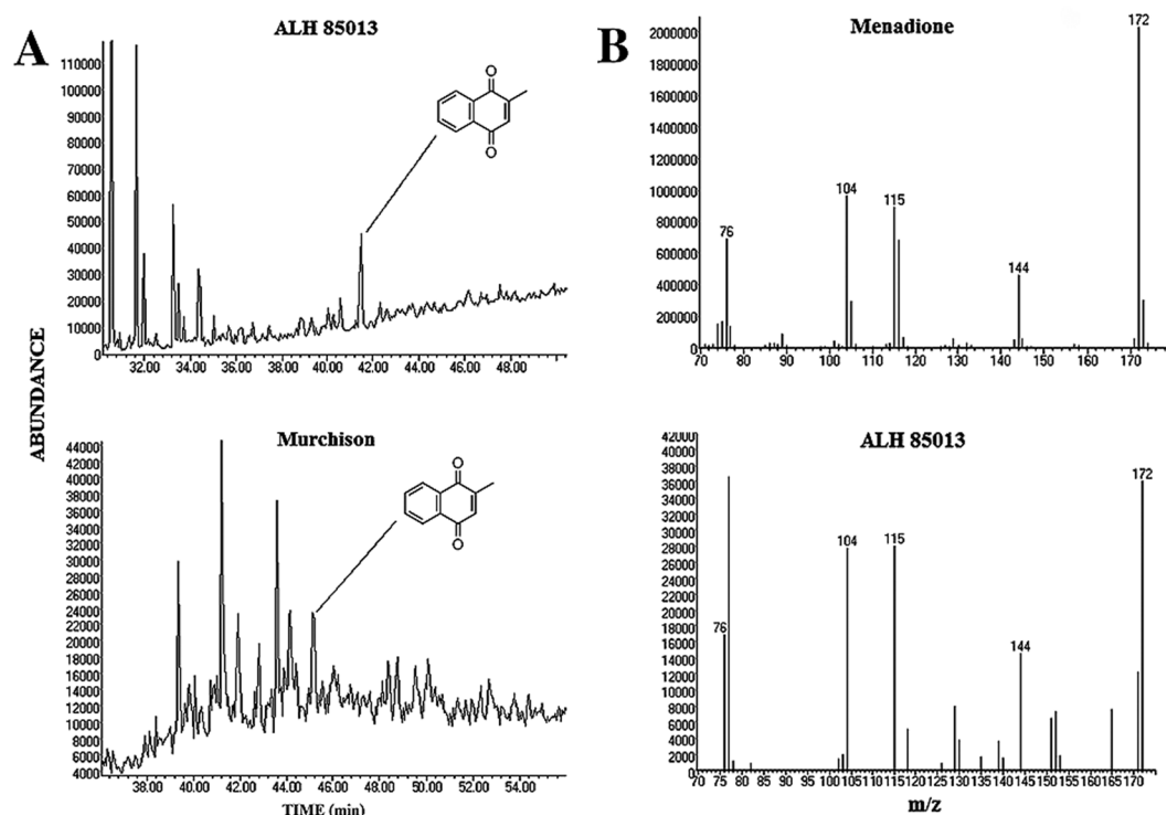
Figure 8. (A) Menadione (2-methylnaphthoquinone) in the ALH 85013 and Murchison meteorites. Traces represent single ion searches for the molecular ion ( m/z 172) of 2-methylnaphthoquinone. (B) Mass spectra of menadione (2-methylnaphthoquinone) and corresponding compounds from ALH 85013. The mass spectrum of ALH 85013 was obtained in SIM mode. Additional fragments are due to co-elution of other meteoritic compounds. The Murchison and ALH 85013 GC temperature programs were different, hence the difference in the retention times of menadione (see Methods section).
