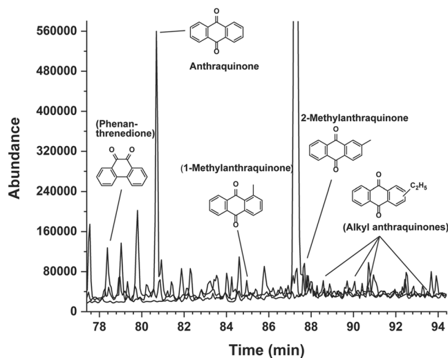
Figure 6. Quinones in the Murchison meteorite. Three individual traces are superimposed that represent single ion searches for the masses (molecular ions) of indicated quinones: m/z 208, anthraquinone (9,10-anthracenedione) and phenanthrenequinone (9,10-phenanthrenedione); m/z 222 (2-methylanthraquinone and isomer); m/z 236 (dimethyl anthraquinone isomers). Compounds in parentheses are tentative: the remaining compounds are definite identifications having GC retention times (x-axis) that match those of authentic standards. The mass spectra of phenanthrenequinone and 1-methylanthraquinone are exact matches of the mass spectra of the corresponding compound in the NIST (National Institute of Standards and Technology) mass spectral database, and the mass spectra of the alkyl anthraquinones are similar to those analyzed laboratory standards of dimethyl or ethyl (i.e., C_2H_5 ) anthraquinone derivatives.
