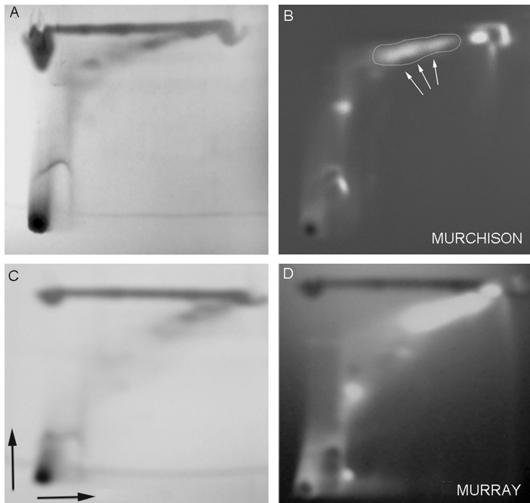
Figure 5. Purifying meteorite extracts by thin layer chromatography. Approximately 0.5–1 mg of Murray and Murchison meteorite samples dissolved in chloroform was spotted at the origin of silica gel TLC plates, then developed with 4:1 hexane:diethyl ether and chloroform in the x and y dimensions respectively (black arrows). (A) Shows the Murchison plate exposed to short wave UV light (254 nm), and (B) shows the same plate exposed to long wave UV light that excited fluorescence (~360 nm). The circled area (white arrows) was scraped and eluted for analysis by mass spectrometry. (C) Shows the Murray plate exposed to short wave UV light, and (D) shows the same plate exposed to long wave UV light.
