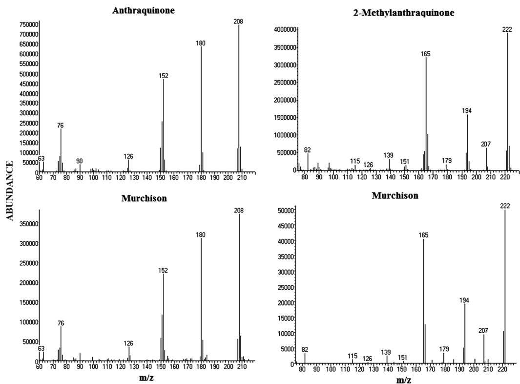
Figure 7. Mass spectra of anthraquinone and 2-methylanthraquinone and corresponding compounds from the Murchison meteorite. The two upper spectra show standards, and the lower spectra were from specific peaks in the GC chromatogram. The mass spectrum of Murchison's 2-methylanthraquinone was obtained in selected ion monitoring (SIM) mode. In SIM, only a limited number of masses (mass-to-charge) are detected, which increases sensitivity.
