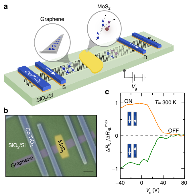
Figure 1 | MoS 2 /graphene vdWh. (a) Schematics of graphene/MoS 2 heterostructure channel with FM source (S) and drain (D) contacts. This structure allows spin injection into graphene from the source (S), diffusive spin transport in the graphene/MoS 2 channel, spin manipulation by a gate voltage and detection of spin signal by the drain (D). (b) Coloured scanning electron microscope image of a fabricated device with a CVD graphene/MoS 2 heterostructure channel and multiple FM tunnel contacts of TiO 2 (1 nm)/Co(80 nm) (scale bar, 1 μm). The devices are fabricated on Si/SiO 2 substrate, which is used as a gate electrode for control of the spin polarization in the channel. (c) Gate dependence of the measured NL resistance ( \Delta R_{NL} = \Delta V_{NL}/I ) normalized to the maximum value, showing transistor-like ON/OFF spin signal modulation at room temperature, for parallel and antiparallel magnetization alignments of source and drain.
