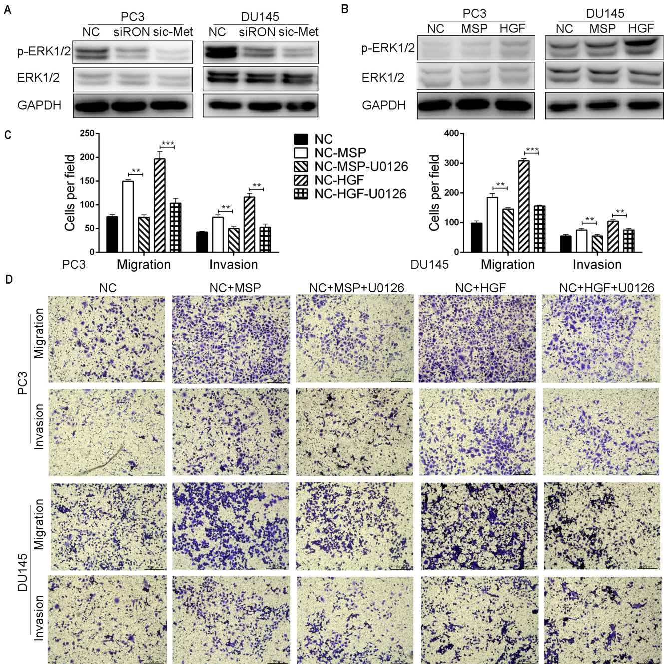
Figure 6. RON and c-Met mediate PCa metastasis via the ERK1/2 pathway. (A) Effect of RON and c-Met on phosphorylation of p-ERK1/2 was analyzed by western blotting. (B) PC3 and DU145 cells were treated with MSP or HGF for 24 h. Level of p-ERK1/2 was detected by western blotting. (C and D) Migration and invasion assays were carried out in the PC3 and DU145 cells following treatment with MSP, HGF and U0126 for 24 h (magnification, \times 200 ). Each experiment was performed in triplicate. ** P < 0.01 , *** P < 0.001 .
