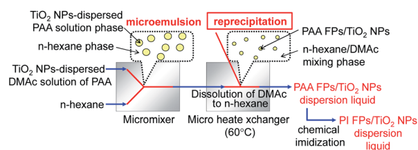
Fig. 1 Schematic diagram of the fabrication process for PI FPs/TiO 2 NPs using a multistep microfluidic system.
