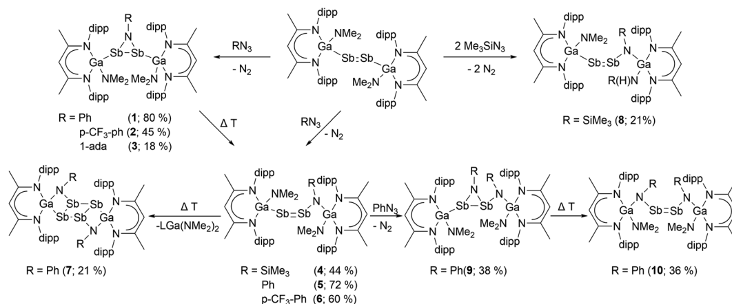
Scheme 2 Azadistibiranes 1–3 and distibenes 4–6 formed by cycloaddition reactions of distibene [\text{L}(\text{Me}_2\text{N})\text{GaSb}]_2 with organoazides. 5 dimerizes to cyclotetrastibane 7 upon thermal treatment and reacts with a second equivalent of \text{PhN}_3 to 9 , which isomerizes to 10 upon heating.
