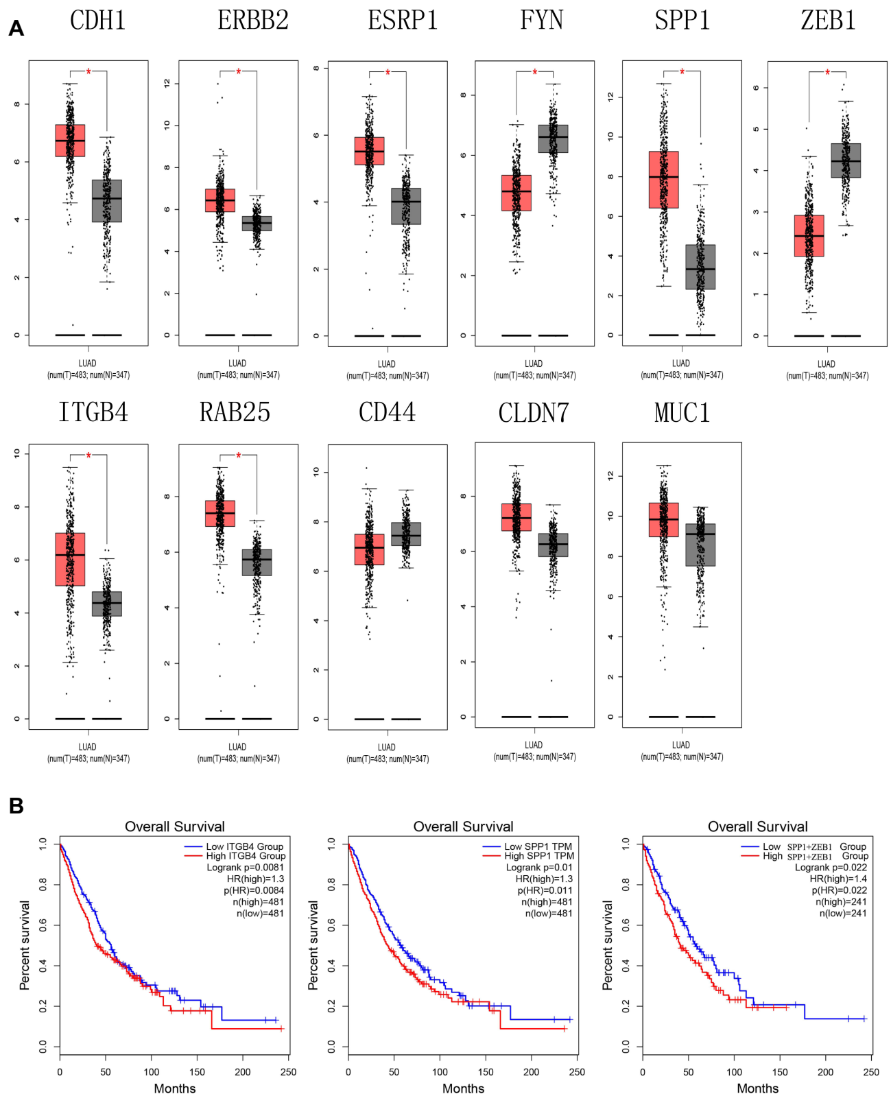
Figure 3 (A) The expression level of hub genes in lung adenocarcinoma and normal tissues in GEPIA ( ^*P < 0.01 ). (B) Survival analysis. Expression level of SPP1 and ITGB4 was related to the overall survival of LUAD and LUSC patients ( P < 0.05 ), expression level of SPP1 + ZEB1 was related to overall survival of LUAD and LUSC patients ( P < 0.05 ).
