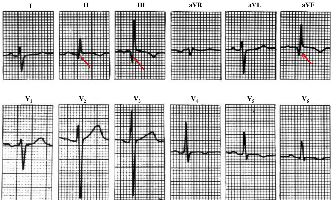
Fig. 3. QRS axis +115^\circ , I and aVL rS; III qR; II, III and aVF qR with inferoapical post-ischemic T wave; V_2 – V_3 deep S waves. LPFB and inferior MI accounted for Q waves in leads II, III and aVF (arrows). However, the R-wave amplitude in these leads is increased after LPFB but decreased after inferior MI. The mean QRS axis in the FP was shifted toward the vertical in LPFB but little changed or slightly shifted away from the vertical in inferior MI.
