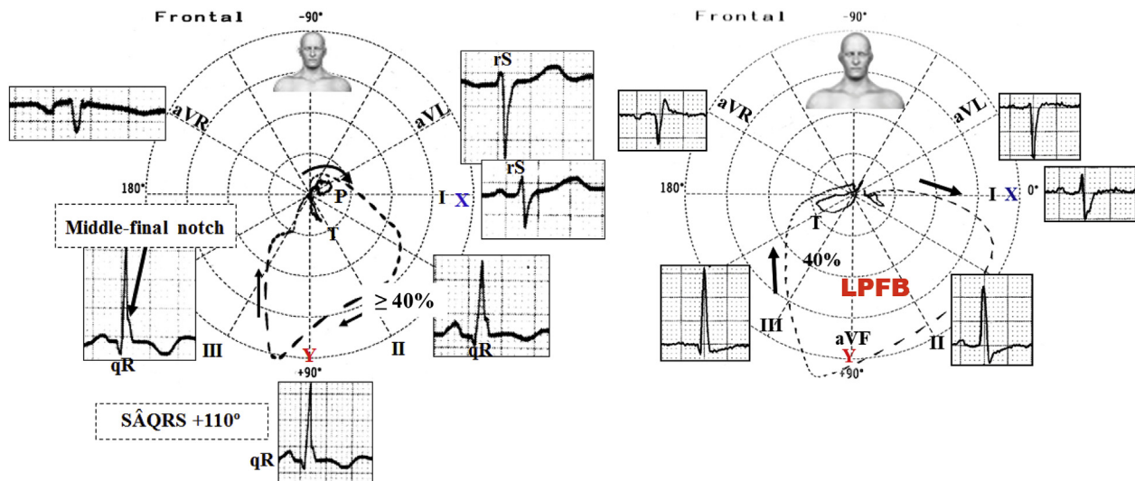
Fig. 15. ECG/VCG correlation in case of isolated LPFB (A) and LPFB associated with RBBB (B).
