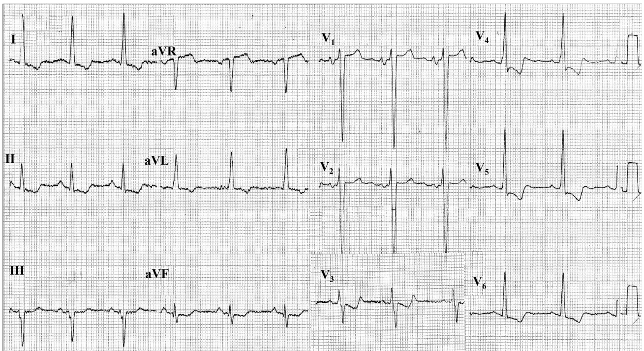
Fig. 6. ECG performed before the percutaneous septal ablation. Clinical diagnosis: obstructive hypertrophic cardiomyopathy with a gradient in LVOT of 80 mmHg and NYHA IV, even with medication. ECG diagnosis: left atrial enlargement + left ventricular hypertrophy (LVH) with strain.
