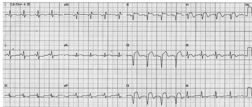
Fig. 14. ECG after percutaneous coronary intervention, RBBB disappears, anterior transmural MI, ST segment elevation from V1 to V4, negative T wave in left precordial leads.
