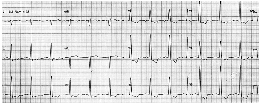
Fig. 10. Right axis deviation (QRS axis in +115^\circ ), rS pattern in leads I and aVL, tall R waves in lead III > RII, and qR pattern (embryonic q) in lead III. This ECG pattern in the limb leads, in the absence of clinical and echocardiographic evidence of RVH, lateral infarction and/or vertical heart associated with significant left ventricular hypertrophy, suggests LPFB. In the chest leads, prominent anterior QRS forces: R wave in V_2 > 15 mm. In the absence of RVH, laterobasal MI, RBBB, pre-excitation with a posterior anomalous pathway, hypertrophic cardiomyopathy, endomyocardial fibrosis, muscular dystrophy, and dextroposition, strongly suggests LSFB.
