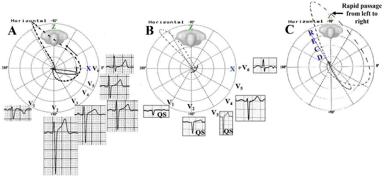
Fig. 16. A: Isolated LPPB in the HP; B: Type C RVH in the HP in a man with severe COPD; C: right posterior subdivision block in a healthy individual.
