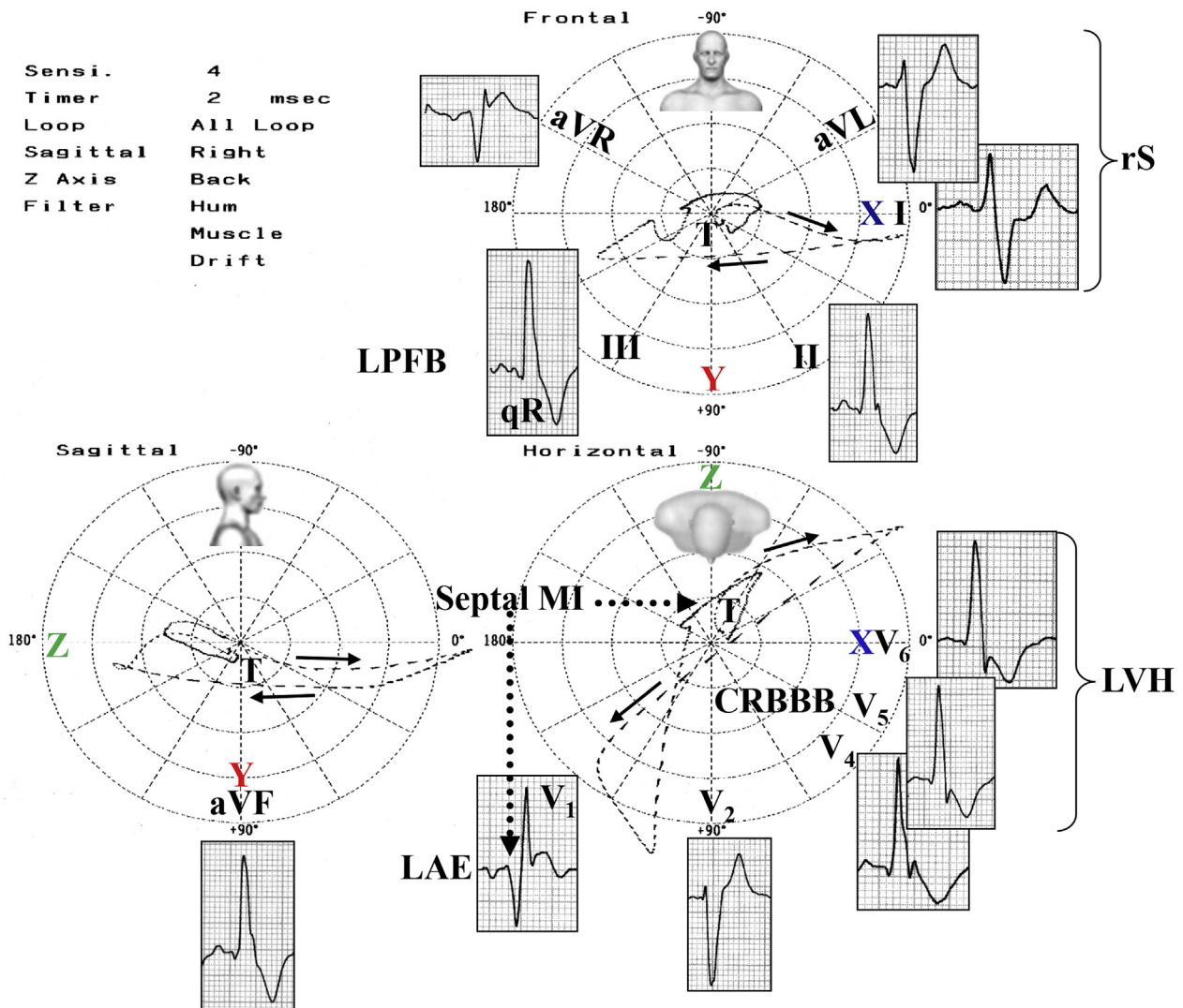
Fig. 7. ECG/VCG correlation immediately after percutaneous procedure. ECG/VCG: LPFB + acute septal MI + LVH + RBBB.
