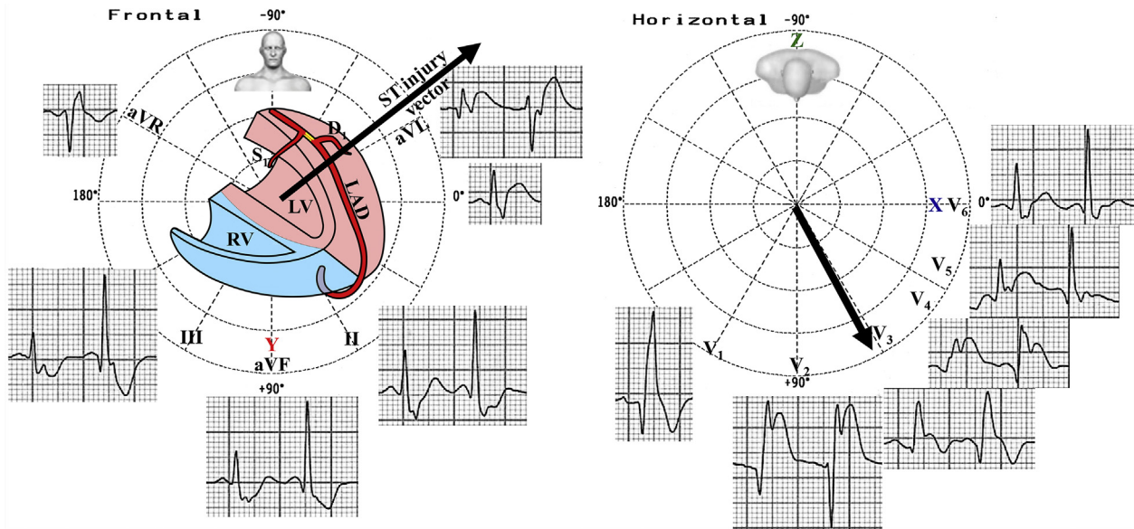
Fig. 12. ECG/VCG correlation in the FP and HP.
