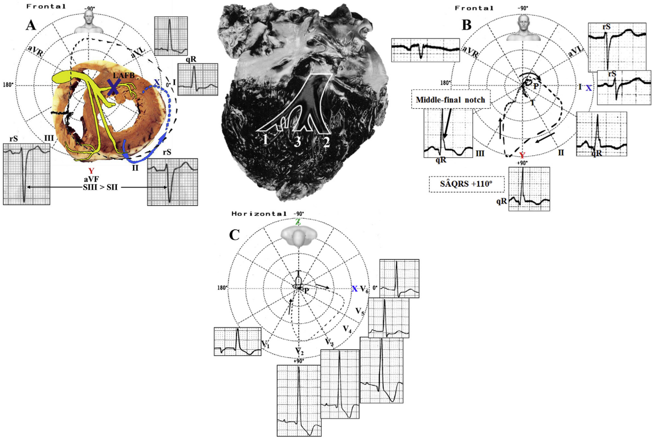
Fig. 1. LAFB (Fig. 1-A) causes left axis deviation in the frontal plane (usually between -45^\circ and -90^\circ ); LPFB (Fig. 1-B) causes right axis deviation in the frontal plane (QRS axis \approx +120^\circ , between +80^\circ and +140^\circ ); while left septal fascicular block (Fig. 1-C) causes prominent anterior QRS forces in the horizontal plane.
