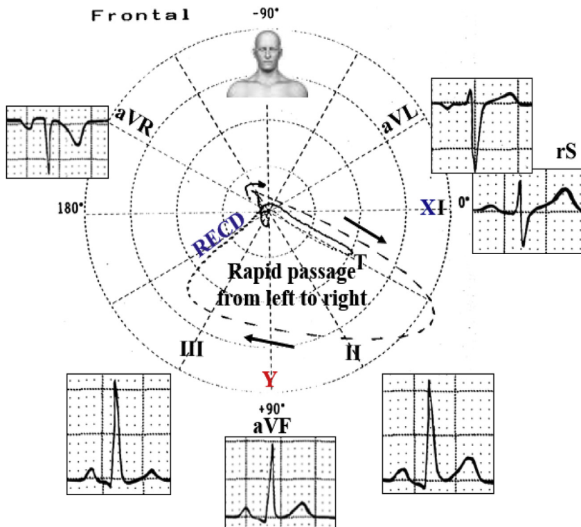
Fig. 19. ECG/VCG correlation: blockage of the inferior fascicle of the RBB.
