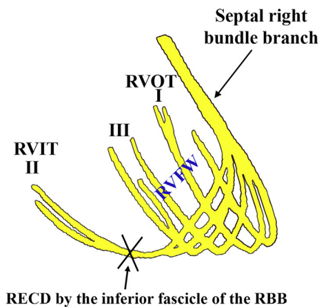
Fig. 17. Outline of the inferior divisional block in RVIT (RECD type II) [23,55,56]. RVIT: right ventricular inflow tract; RVOT: right ventricular outflow tract; RVFW: right ventricular free wall.
