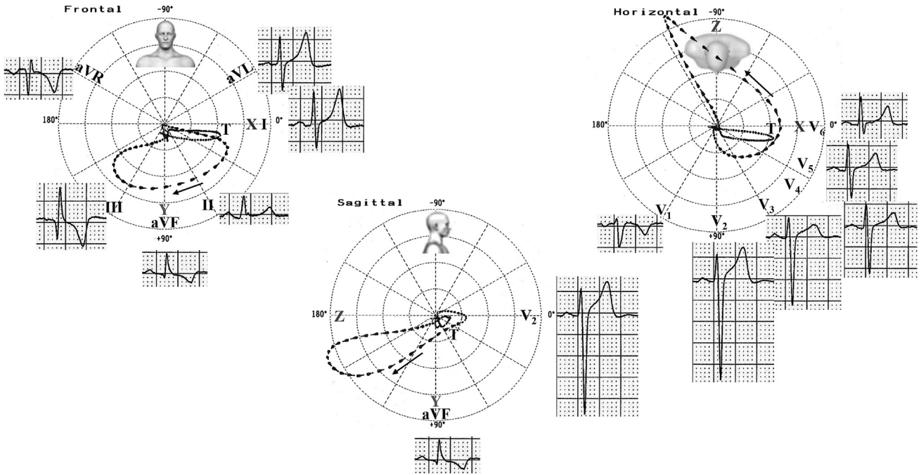
Fig. 8. VCG/ECG correlation in isolated LPFB.
