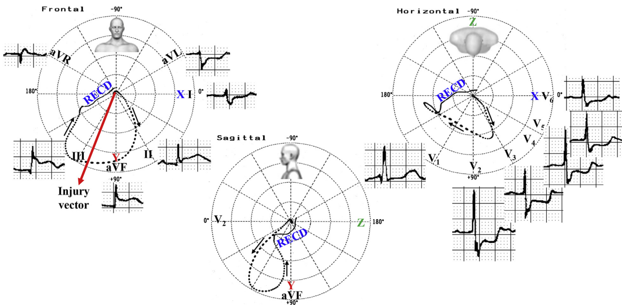
Fig. 2. Example of LPFB + complete RBBB Kennedy type III + hyperacute phase of inferior MI by obstruction of RCA. FP: QRS axis +150^\circ , VCG QRS loop with clockwise rotation and located in inferior quadrants ( >40\% area in inferior right quadrant), injury vector pointed to III suggesting proximal obstruction of RCA, ST segment depression in I and aVL, ST segment elevation (STE) in inferior leads ( STE_{III} > STE_{II} ). HP: QRS loop located in the anterior quadrants, CW rotation, right end conduction delay (RECD) in the right anterior quadrant, complete RBBB Kennedy type III. LSP: all QRS loop located in anterior and inferior quadrants, QRS loop with counterclockwise rotation. Conclusion: LPFB + complete RBBB + acute inferior MI.
