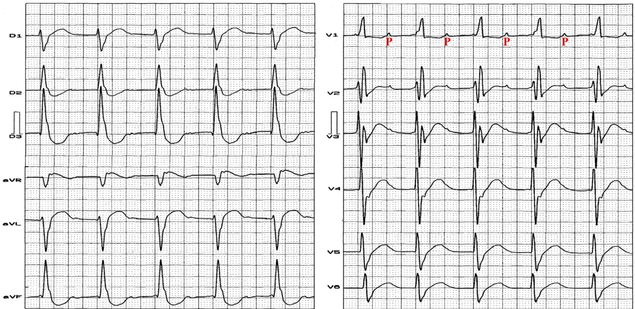
Fig. 5. Clinical features: 85-year-old female. Autopsy diagnosis: Lev's disease. ECG diagnosis: 1st degree AV block + LPFB + RBBB: probable trifascicular block + digitalis effect.
