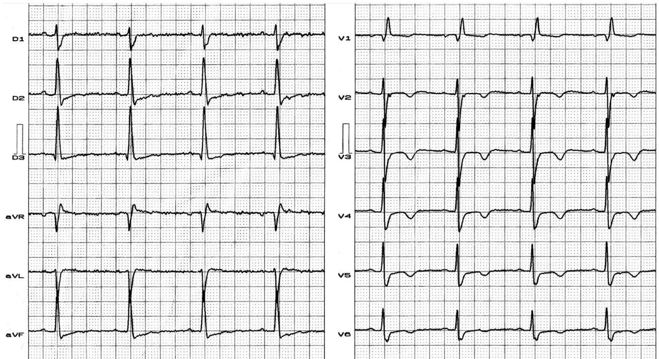
Fig. 9. Typical RBBB pattern associated with LPFB, septal infarction (qR in V1) and anterior ischemia.
