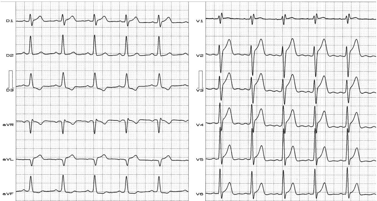
Fig. 18. ECG of a young male athlete with normal heart.
