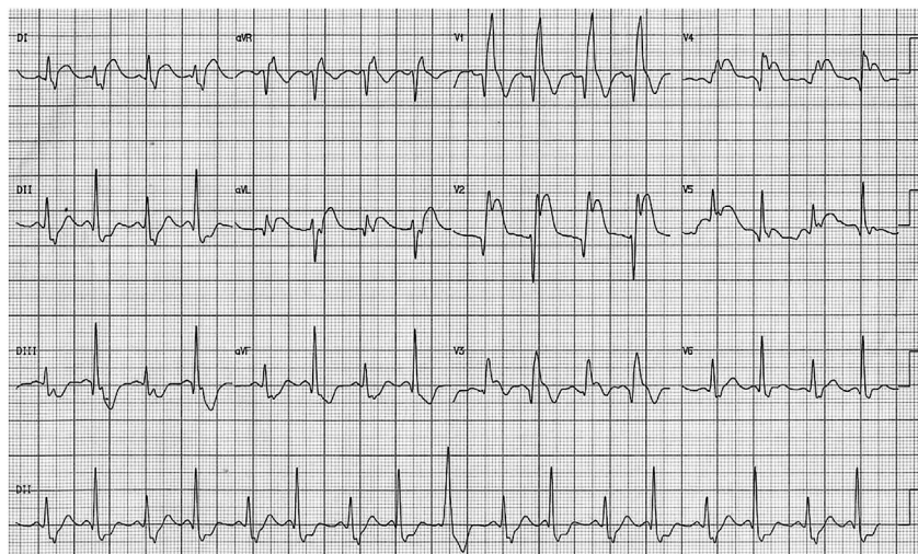
Fig. 10. Right axis deviation (QRS axis in +115^\circ ), rS pattern in leads I and aVL, tall R waves in lead III > RII, and qR pattern (embryonic q) in lead III. This ECG pattern in the limb leads, in the absence of clinical and echocardiographic evidence of RVH, lateral infarction and/or vertical heart associated with significant left ventricular hypertrophy, suggests LPFB. In the chest leads, prominent anterior QRS forces: R wave in V_2 > 15 mm. In the absence of RVH, laterobasal MI, RBBB, pre-excitation with a posterior anomalous pathway, hypertrophic cardiomyopathy, endomyocardial fibrosis, muscular dystrophy, and dextroposition, strongly suggests LSFB.
