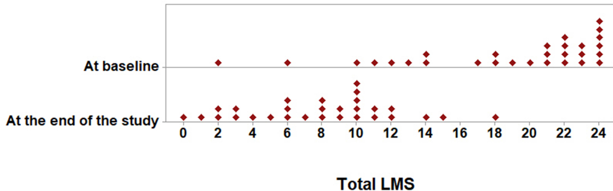
Figure 2 Dot plot of LMS at base line and at the end of the study.
