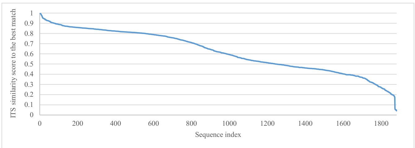
Fig. 20. The ITS similarity scores of the most wanted sequences to their best-match ITS barcodes.
