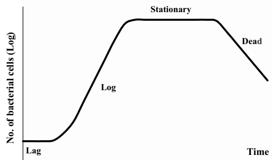
Figure 1. Graphic representation of typical bacterial growth curve in culture medium. When bacteria are introduced into the fresh medium in a closed system, like a test tube, the population of cells always exhibits growth dynamics as follows. Lag phase: bacteria initially adjust to the new environment, so they appear not able to replicate but the cells might grow in volume; Log (exponential) phase: cells start dividing regularly by the process of binary fission. The culture reaches the maximum growth rate, which could be estimated by generation time or doubling time, i.e., the time per generation; Stationary phase: the number of cells undergoing division seems to be equal to that being dead due to the exhaustion of nutrients. Dead phase: bacteria lose the ability to divide and the number of dead cells exceeds that of live cells.
