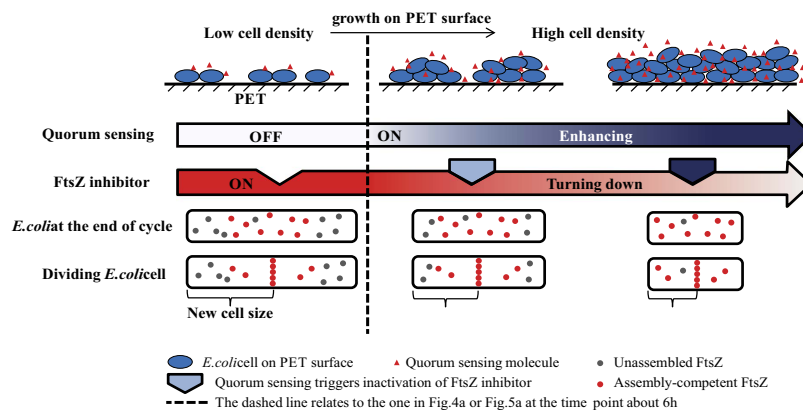
Figure 8. The E. coli cell size control model when growing on PET surfaces.
