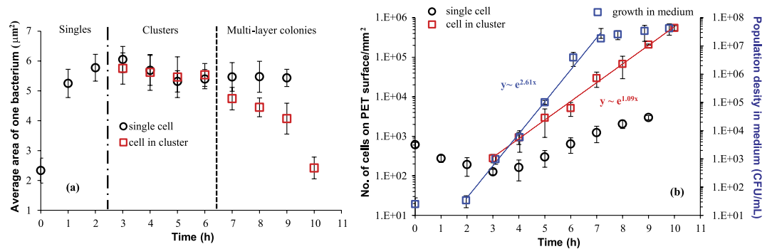
Figure 4. (a) The cell size of bacteria on PET surfaces at each hour interval. (b) The curves of bacterial growth on PET surfaces and in a separate test in LB bulk culture medium (for comparison). The exponential regression fits in the log phase are shown for the bulk and substrate populations. Singles are no longer measured at 10 h since it is difficult to distinguish the single cells from the cells in clusters then.
