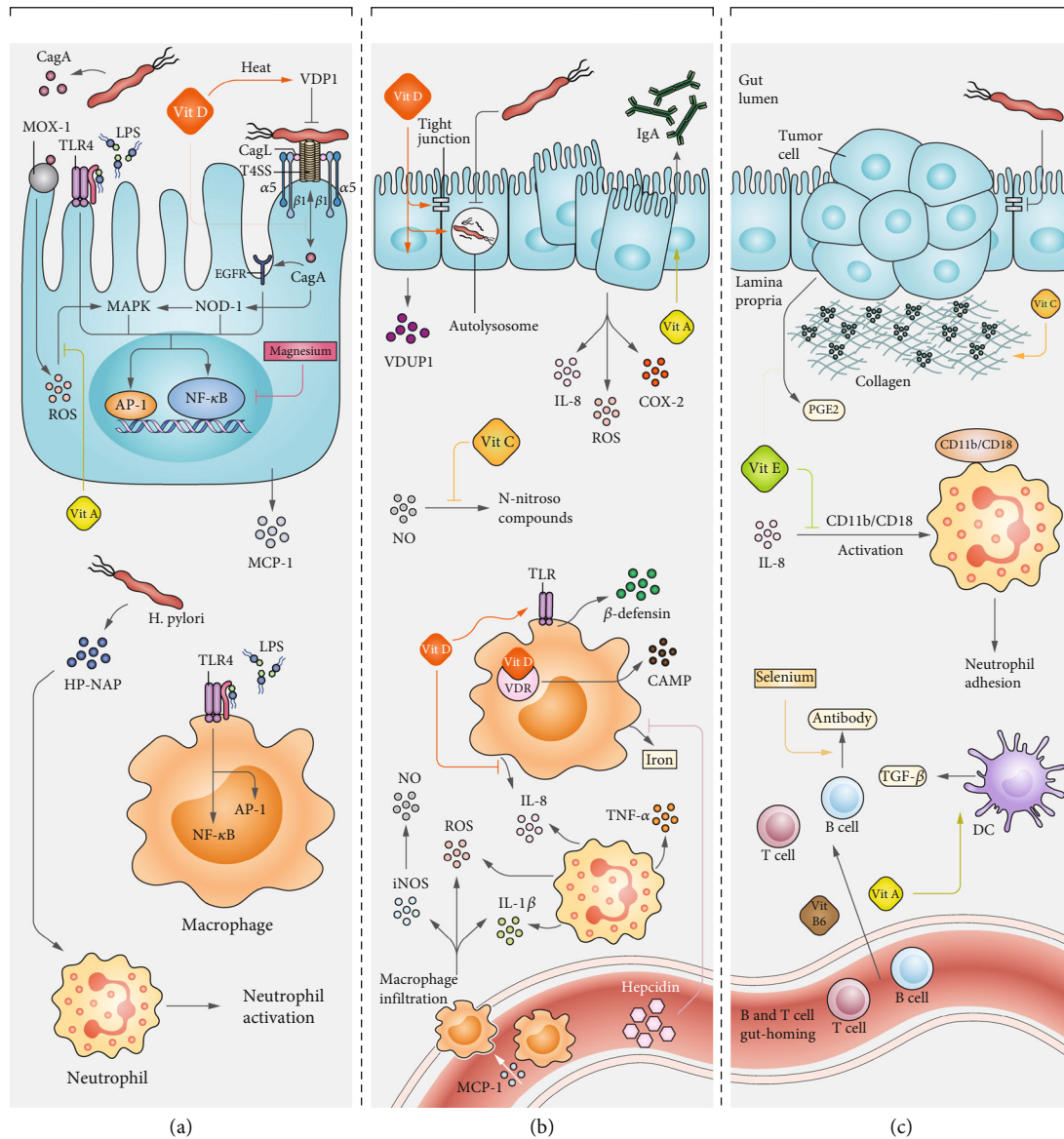
FIGURE 1: The effect of micronutrients on H. pylori pathogenesis. (a) H. pylori can invade epithelial cells and interact with epidermal growth factor receptor (EGFR), toll-like receptor 4 (TLR4), and mitogen oxidase-1 (Mox1), thereby stimulating the activation of transcriptional factors and the production of reactive oxygen species (ROS). H. pylori neutrophil-activating protein (HP-NAP) and LPS lead to neutrophil activation and promotion of macrophage inflammatory responses, respectively. However, vitamin D and A interfere with CagA expression and ROS-mediated mitogen-activated protein kinase (MAPK) activation, respectively. Furthermore, vitamin D3 decomposition product (VDP1) lyses the bacterial cell and inhibits the colonization of H. pylori . Magnesium downregulates the activation of nuclear factor kappa B (NF-κB) and activated protein-1 (AP-1); therefore, suppressing the host inflammatory responses. (b) Neutrophil activation promotes the production of tumor necrosis factor-α (TNF-α), interleukin 8 (IL-8), IL-1β, and ROS. Macrophage chemotactic protein-1 (MCP-1) stimulates the infiltration of macrophages and thereby increases the concentration of inducible nitric oxide synthase (iNOS), IL-1β, and ROS in the gut lamina propria. The infected epithelial cells overexpress proinflammatory cytokines such as cyclooxygenase-2 (COX-2), IL-8, and ROS. The overproduction of hepcidin in the liver, owing to H. pylori infection, interferes with the iron release from the macrophages. Vitamin D and A promote the expression of Vitamin D upregulated protein 1 (VDUP1) and immunoglobulin A (IgA), respectively. Regarding macrophages, vitamin D inhibits IL-8 secretion, increases β-defensin production through TLR activation and provokes the production of cathelicidin antimicrobial peptide (CAMP) by vitamin D receptor (VDR). Vitamin D regulates the reduced function of autolysosome and consequently stimulates H. pylori degradation in gastric epithelial cells. Moreover, this vitamin promotes the gut epithelial barrier by increasing the expression of tight junctions. On the other hand, vitamin C can reduce N-nitroso compound formation from nitric oxide (NO) and thereby inhibits carcinogenesis. (c) As chronic inflammation results in carcinogenesis, vitamin C promotes collagen production and prevents tumor metastasis. On the other hand, vitamin E reduces neutrophil adhesion and the secretion of prostaglandin E2 (PGE2) from tumor cells. Vitamin A and B6 induce B and T cell gut-homing, and selenium provokes the antibody secretion from B cells. Vitamin A is also involved in the production of transforming growth factor-beta (TGF-β) in the dendritic cells (DCs).
