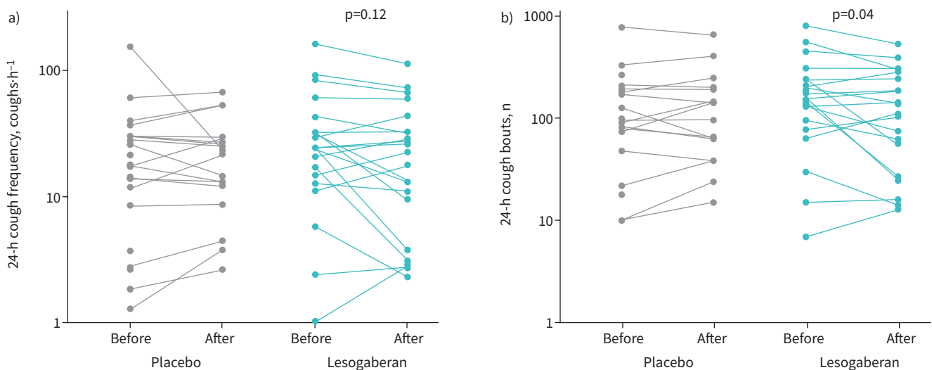
FIGURE 2 a) Cough frequency and b) cough bout data before and after 2 weeks' placebo and lesogaberan treatment. Lesogaberan reduced 24-h cough frequency by 26% ( p=0.12 ) and cough bouts by 31% over placebo ( p=0.04 ).
