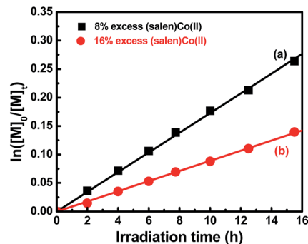
Fig. 4 Kinetic plots for the polymerization of MA with an excess amount of (salen)Co(II) . [MA]_0 = 1.0 M, [MA]_0/[I]_0 = 600/1 . ■ 8% (salen)Co(II) added, conv. = 23%, M_{n,th} = 12\ 500 , M_{n,GPC} = 11\ 600 , M_w/M_n = 1.08 . ● 16% (salen)Co(II) added, conv. = 13%, M_{n,th} = 7380 , M_{n,GPC} = 7370 , M_w/M_n = 1.09 .
