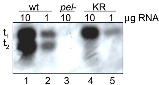
Figure 2 Northern blot analysis of mRNA in CS101 (wt), CS101 sagA/pel::Tn917 ( pel- ) and CS101 sagA/pel::Tn917 kidney-recovered (KR). Bacteria were grown overnight at 37°C, 10% CO 2 in Todd-Hewitt Yeast extract broth. RNA was extracted and 10 μg or 1 μg of total RNA was loaded on a 1.0% MOPS-formaldehyde agarose gel. After blotting the RNA to a charged nylon filter, sagA/pel RNA was detected using a biotinylated probe. t 1 and t 2 represent the two transcripts detected in the wild type strain. Only t 1 was detected in the KR variant.
