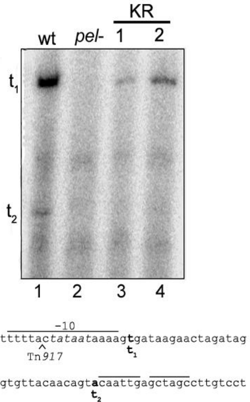
Figure 3 Primer extension analysis of sagA/pel from wild type, sagA/pel mutant and kidney-recovered strains. Bacteria were grown overnight at 37°C with 10% CO 2 in THY broth. RNA was extracted and sagA/pel was detected using a primer extension assay and sagA/pel -specific primers. Equal amounts of RNA were loaded in each lane. Lane 1, RNA isolated from a wild type CS101 strain. Lane 2, RNA from an isogenic sagA/pel::Tn917 mutant. Lanes 3 and 4, RNA isolated from 2 different KR variants of the sagA/pel mutant. The larger sagA/pel transcript is indicated as t 1 , the smaller as t 2 . The DNA sequence in the lower part of the figure is from the region around the sagA/pel promoter. These represent bases 598514–598593 in the S. pyogenes genome [43]. The bases in italics are the putative -10 region of the sagA/pel promoter. The overlined regions are 16, 6 and 6 base inverted repeats. The bold letters are the 5'-ends of the t 1 and t 2 transcripts as determined by primer extension. The position of the Tn917 insertion is indicated by the ^ symbol. Note that the site of insertion is slightly different from what was previously reported [4]. The t 2 transcript was not detected in the KR variants even at longer exposures.
