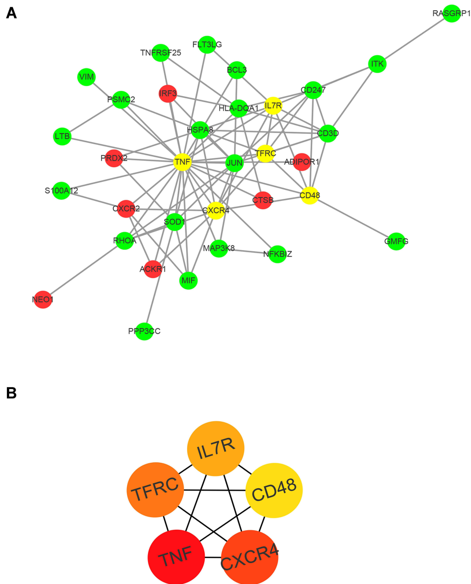
Figure 4 PPI network of identified DEIRGs constructed using Cytoscape software. (A) DEIRGs in the INRs vs IRs . Red nodes represent up-regulated genes, green nodes represent down-regulated genes, and yellow nodes represent hub genes in INRs. (B) The top module and the top five DEIRGs between INRs and IRs. Abbreviations: DEIRG, differentially expressed immune-related genes; INRs, immunological non-responders; IRs, immunological responders.
