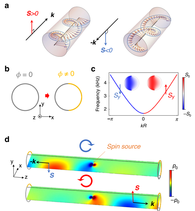
Fig. 1 Spin angular momentum in waveguide with symmetry-breaking boundary conditions.
