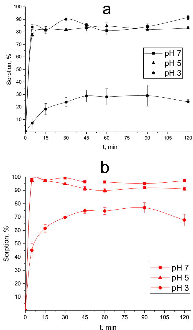
Figure 3. The influence of pH of the initial solution to the ^{68}\text{Ga} sorption onto nanodiamonds (ND) (a) and their oxidized forms (ND-COOH) (b) at m/V ratio of 100 \mu\text{g}/\text{mL} and at 25 ^{\circ}\text{C} .
