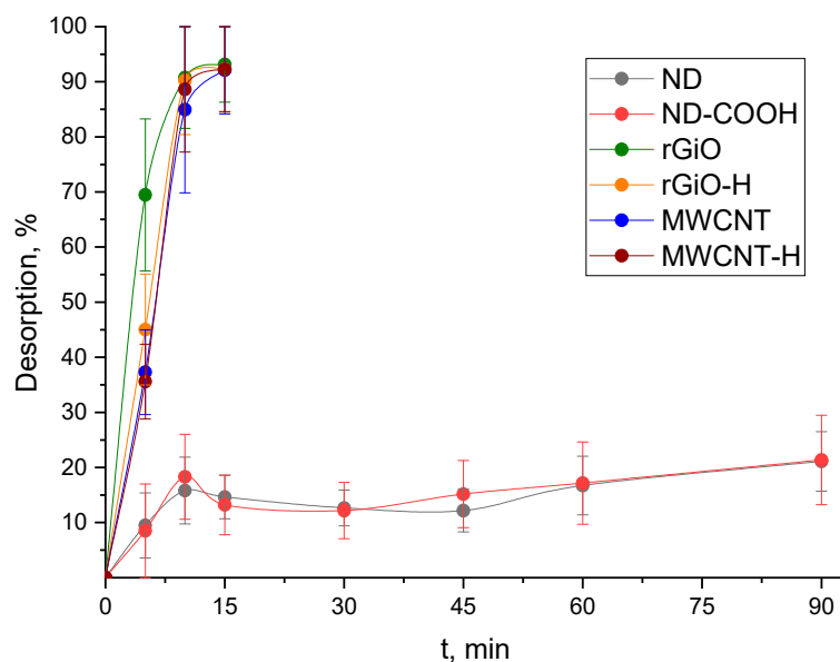
Figure 4. Desorption of ^{68}\text{Ga} from studied CNMs (100 \mu\text{g}/\text{mL} ) by the solution of 40 g/L bovine serum albumin (BSA) in phosphate-buffered saline (PBS) at 25 °C.
