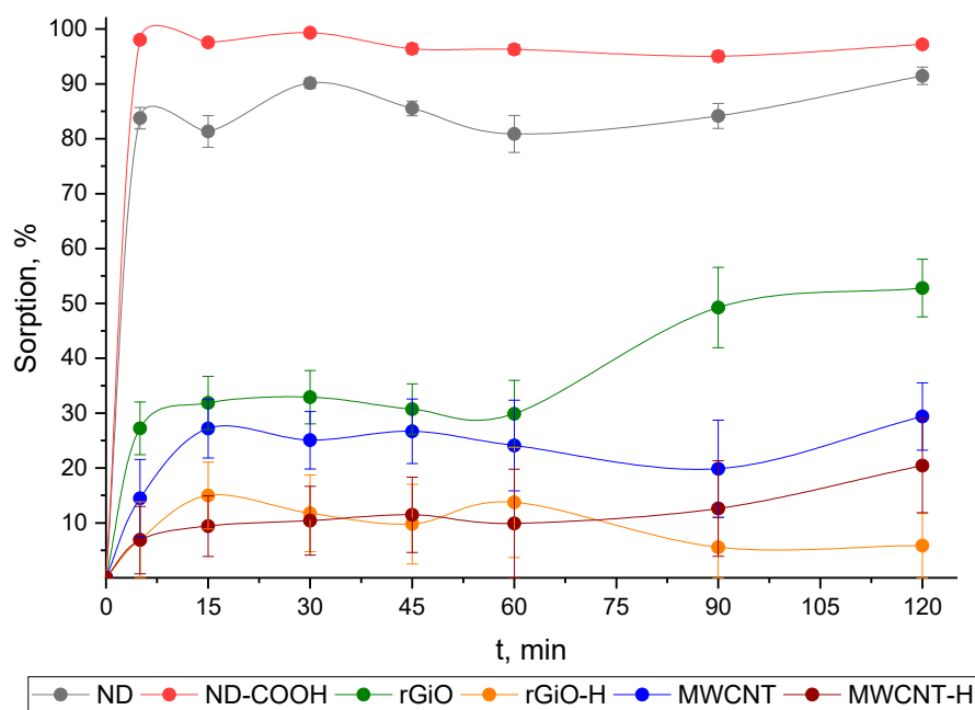
Figure 1. Sorption kinetics of ^{68}\text{Ga} by studied CNMs from an aqueous solution with a pH 7 at m/V ratio of 100 \mu\text{g}/\text{mL} and 25 ^{\circ}\text{C} .
