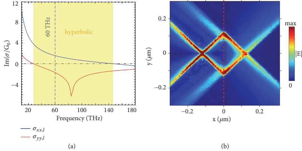
FIGURE 4: Negative refraction of hyperbolic polaritons supported by naturally anisotropic 2D materials. (a) Imaginary part of surface conductivity of anisotropic 2D material in the left region. In (2), we set n = 3 \times 10^{13} \text{ cm}^{-2} , m_x = 0.2m_0 , m_y = m_0 , \omega_x = 1 \text{ eV} , \omega_y = 0.35 \text{ eV} , \tau = 0.4 \text{ ps} , s_x = 1.7s_0 , and s_y = 3.7s_0 , where s_0 = e^2/4\hbar and m_0 is the free-electron mass. (b) Distribution of electric field |\vec{E}| excited by a dipole source at 60 THz. The red dashed line represents the boundary between left/right regions. For the right region, we have \sigma_{xx,r} = \sigma_{yy,l} and \sigma_{yy,r} = \sigma_{xx,l} .
