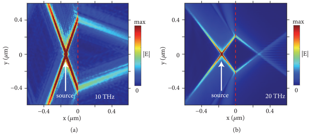
FIGURE 3: All-angle negative refraction of hyperbolic polaritons (a) at 10 THz and (b) at 20 THz. The other parameters are the same as that in Figure 1(c). The values of anisotropic surface conductivity for graphene metasurfaces are highlighted by grey dashed lines in Figure 2(a).
