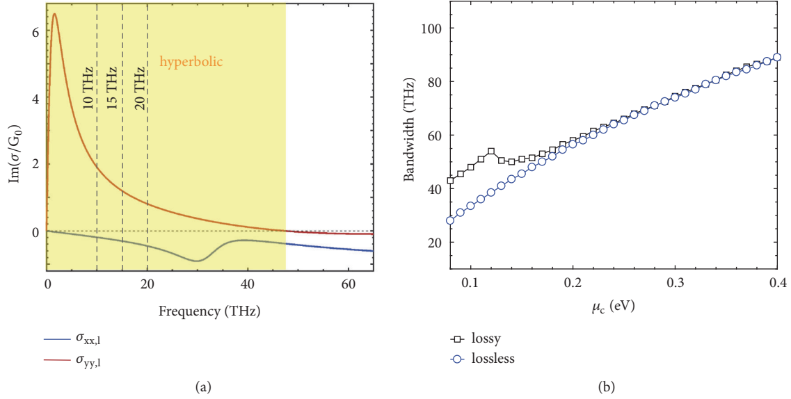
FIGURE 2: Broadband all-angle negative refraction of hyperbolic polaritons. (a) Imaginary part of surface conductivity of graphene metasurface, created by nanostructured graphene as shown in the left region of Figure 1(a) and having an effective anisotropic surface conductivity of \bar{\sigma}_l = [\sigma_{xx,l}, \sigma_{yy,l}] . The graphene metasurface supports hyperbolic plasmon polaritons when \text{Im}(\sigma_{xx,l}) \cdot \text{Im}(\sigma_{yy,l}) < 0 , i.e., the region highlighted by yellow. The chemical potential of graphene is \mu_c = 0.1 eV. (b) Bandwidth of graphene metasurface having \text{Im}(\sigma_{xx,l}) \cdot \text{Im}(\sigma_{yy,l}) < 0 , as a function of the chemical potential. The phenomenon of all-angle negative refraction of hyperbolic polaritons can happen within this bandwidth. The constant G_0 = e^2/4\hbar is the universal optical surface conductivity.
