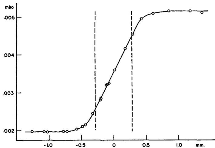
FIG. 7. Conductance of the measuring cell, with a glass rod in place of the squid axon. The rod is introduced between the electrodes and is moved to the right so its left end goes through the electrode region. The electrode boundaries are given by the broken lines and the abscissae are distances in millimeters between the left end of the rod and the center of the electrodes.
