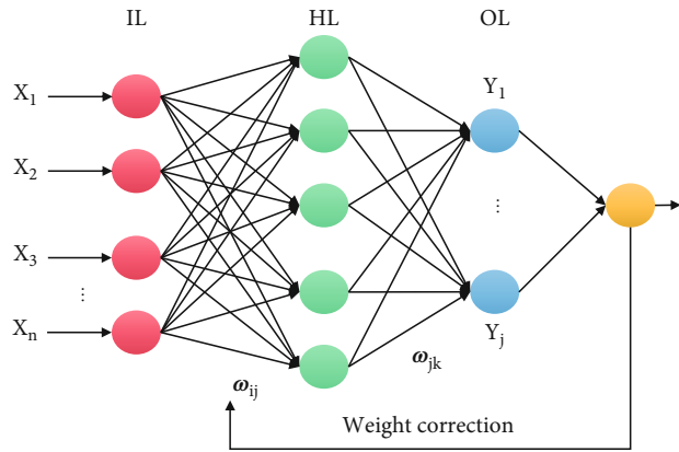
FIGURE 2: BPNN structure.
