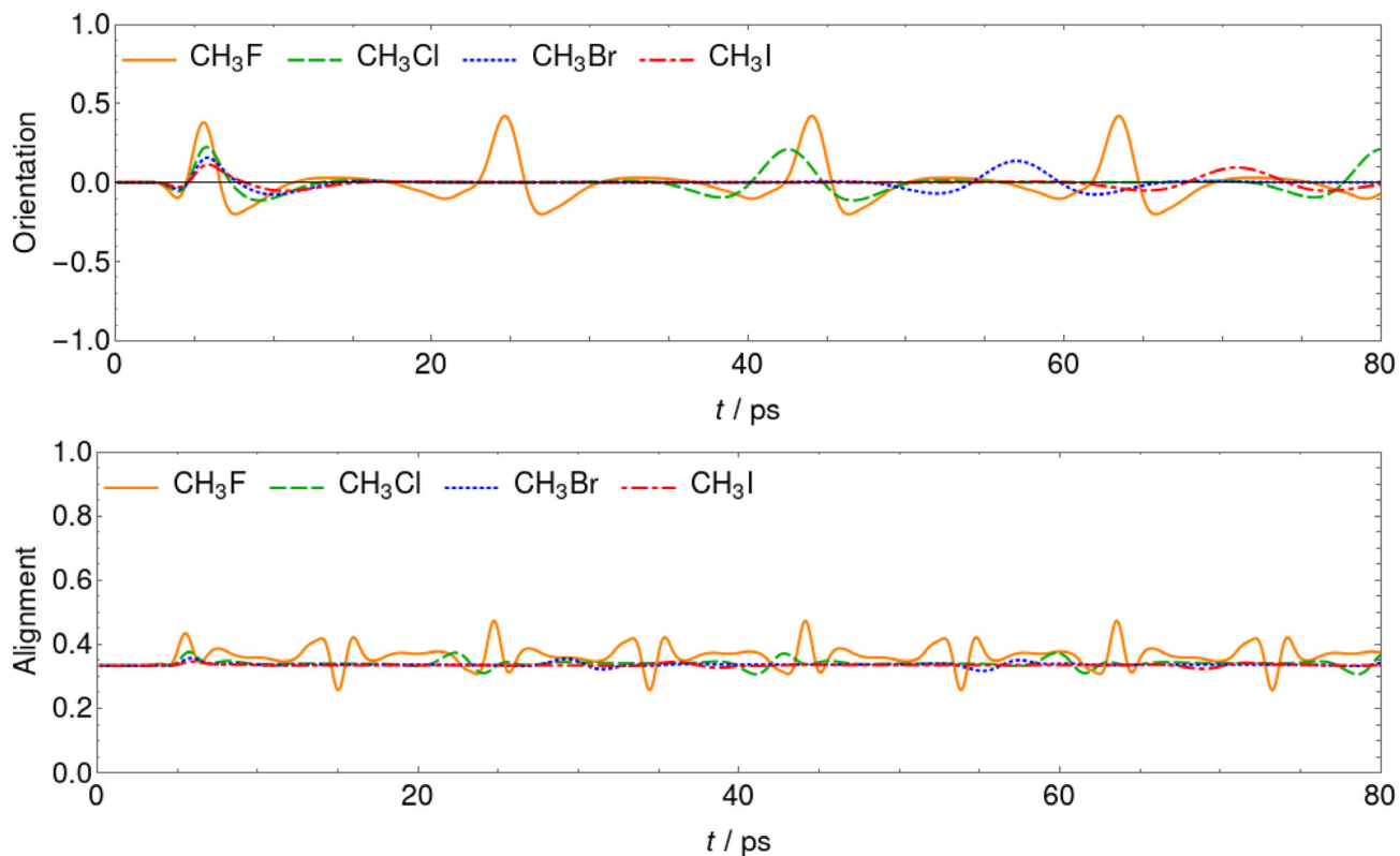
FIGURE 9 Alignment and orientation dynamics of the CH 3 X molecules following a THz-pulse excitation with pulse parameters of T/K = 5 , \nu/\text{THz} = 0.333 , \text{FWHM}/\text{fs} = 2000 , I/\text{TW cm}^{-2} = 5 \times 10^{-4} , pulse position at 5 ps, and \text{CEP} = \pi/2
