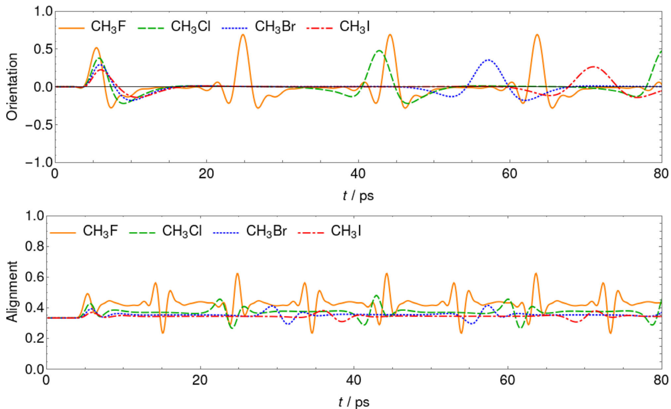
FIGURE 8 Alignment and orientation dynamics of the CH 3 X molecules following a THz-pulse excitation with pulse parameters of T/K = 5 , \nu/\text{THz} = 0.25 , \text{FWHM}/\text{fs} = 2000 , I/\text{TW cm}^{-2} = 5 \times 10^{-4} , pulse position at 5 ps, and \text{CEP} = \pi/2
