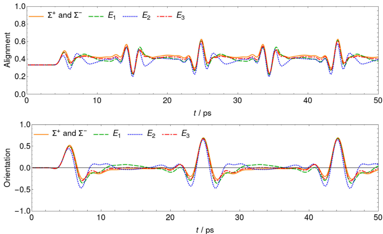
FIGURE 13 Role of symmetry in the A&O dynamics of \text{CH}_3\text{F} (see text for details). Pulse parameters: T/K = 5 , \nu/\text{THz} = 0.25 , \text{FWHM}/\text{fs} = 2000 , pulse position is 5 ps, I/\text{TW cm}^{-2} = 5 \times 10^{-4} , and \text{CEP} = \pi/2
