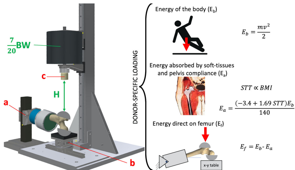
FIGURE 1. On the left-hand side, the drop tower machine. The aluminium plate and the distal hinge joint (a), the low-friction x - y table (b), the hammer equipped with the impact load cell (c) are displayed. On the right-hand side, a schematic representation of the process used for determining the drop height and mass including the jack-knife model (top), the energy balance at the hip (centre) and the schematic representation of the simulated impact on the femur (bottom).
