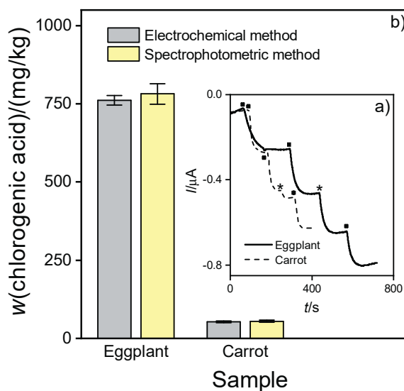
Fig. 1. Images show: a) amperograms obtained with the electrochemical biosensor in 600 \mu M H_2O_2 and 0.1 M phosphate buffer (pH=5), after the addition of 0.85 \mu M chlorogenic acid ( \bullet ) or sample ( * ): an aliquot of 10 \mu L fresh-cut eggplant (solid black line) and 20 \mu L carrot (dashed black line) extracts. Working potential: -200 mV, and b) polyphenolic compound content in fresh-cut eggplant and carrot extracts by electrochemical and spectrophotometric methods
