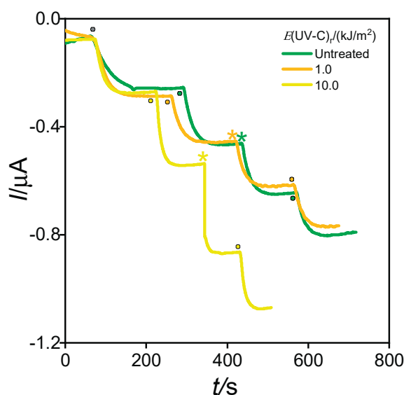
Fig. 3. Amperograms obtained with the electrochemical biosensor in 600 \mu M H_2O_2 and 0.1 M phosphate buffer (pH=5) after the addition of 0.85 \mu M chlorogenic acid (●) or 10 \mu L of fresh-cut eggplant extract (*) (0 storage days) irradiated with different UV-C light intensities: untreated (green line), E_r=1.0 orange line) and 10.0 kJ/m 2 (yellow line). Working potential: -200 mV
