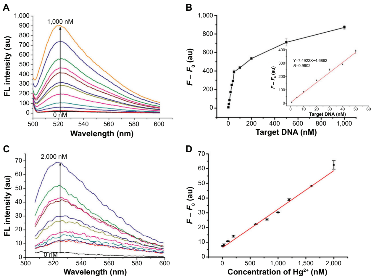
Figure 6 Fluorescence spectra (A, C) and the changeable fluorescence intensities (B, D) towards different concentrations of MDR1 gene (A, B) and Hg^{2+} (C, D).
