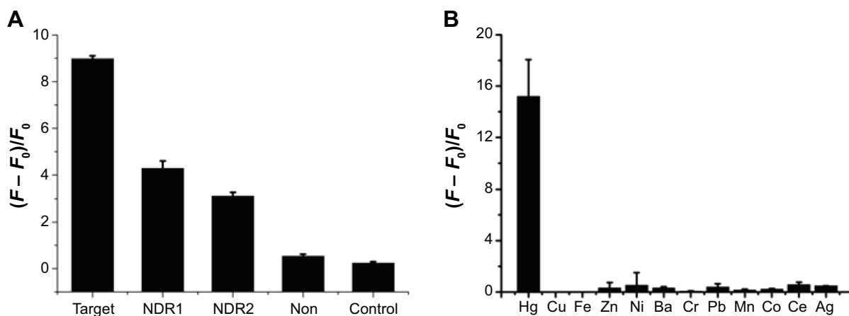
Figure S2 (A) Fluorescence intensities for 8 μL SGI, 50 nM CP, and 2 μg/mL GO upon addition of 20 nM target, one-based mismatch, three-based mismatch, non-complementary MDR1 gene, and without any target. (B) Selectivity evaluation of 8 μL SGI, 80 nM MC, and 2 μg/mL GO toward 2,000 nM Hg 2+ and other ions.
