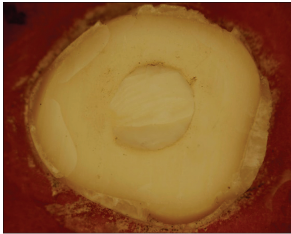
Figure 5: Cohesive failure
