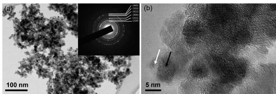
Fig. 3 TEM images of the \text{Fe}_3\text{O}_4@SiO_2\text{-APTESFe}_2L^{\text{DAR}} catalysts at lower (a) and higher (b) magnifications. The inset in (a) is a selected-area electron-diffraction pattern acquired from the area indicated in (a) and indexed according to the cubic spinel structure (Space group Fd\bar{3}m ). The black arrow in (b) shows an iron-oxide nanoparticle, while the white arrow shows an amorphous \text{SiO}_2 layer.
