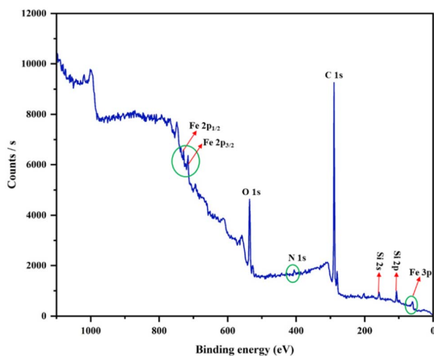
Fig. 4 X-ray photoelectron spectroscopy (XPS) spectrum of catalyst ( \text{Fe}_3\text{O}_4@SiO_2\text{-APTES-Fe}_2L^{\text{DAR}} ).
