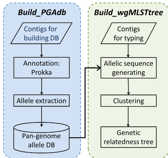
Figure 1. The schematic work flow of PGAdb-builder.
