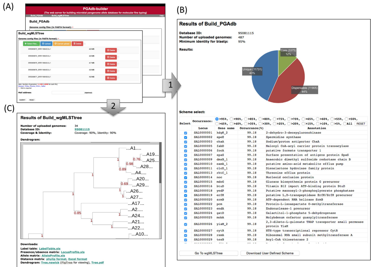
Figure 2. The features of the PGAdb-builder server. (A) Input page of the Build_PGAdb (right panel) and the Build_wgMLSTtree (left panel). (B) Output page of the Build_PGAdb . (C) Output page of the Build_wgMLSTtree .
