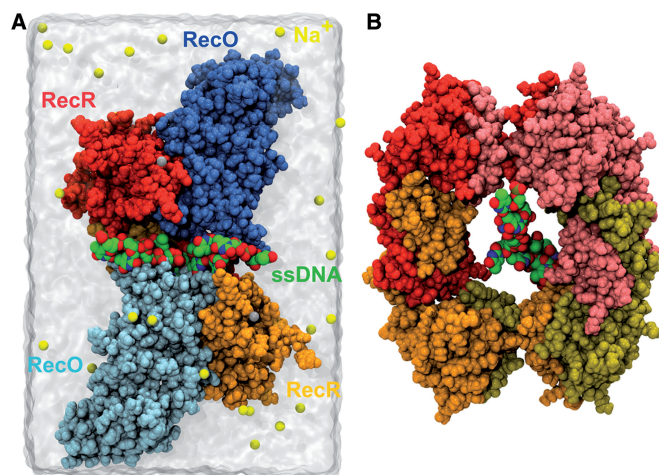
Figure 6. MDs simulations set-up. (A) Initial setup of the drRecOR/ssDNA complex immersed in a water box. Yellow and gray spheres depict sodium counter-ions and zinc ions, respectively. For clarity purposes, only two RecR subunits are shown. (B) View of the initial position of the 10-thymine ssDNA in the central cavity of the drRecR tetrameric ring. The RecO and RecR chains are colored as in Figure 2.
