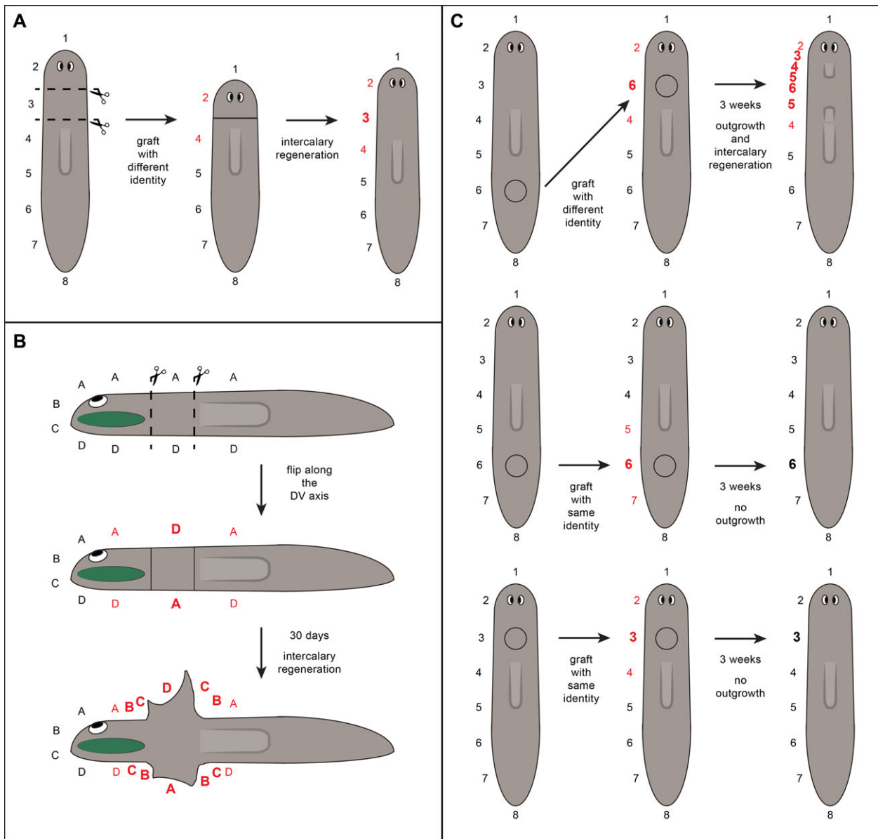
Figure 2. Juxtaposition of tissues with different positional identities induces intercalary regeneration. Differential expression of position control genes, biophysical properties and presence of different tissues manifest positional identities along the AP (1–8; 1 is most anterior, 8 is most posterior) and DV (A–D; A is dorsal, D is ventral) axes. (A) Grafting head fragments onto pharyngeal areas induces intercalary regeneration of the missing anterior areas (Reddien & Sanchez Alvarado 2004). (B) Reversing the orientation of a prepharyngeal graft along the DV axis induces generation of ectopic outgrowths (Kato et al. 1999). (C) Grafting posterior fragments into anterior areas induces development of outgrowths and regeneration of new pharynges on either side of the outgrowth (Kobayashi et al. 1999). In contrast, grafts from posterior tissues into tail areas or anterior tissues into prepharyngeal areas did not induce formation of outgrowths (Kobayashi et al. 1999).
