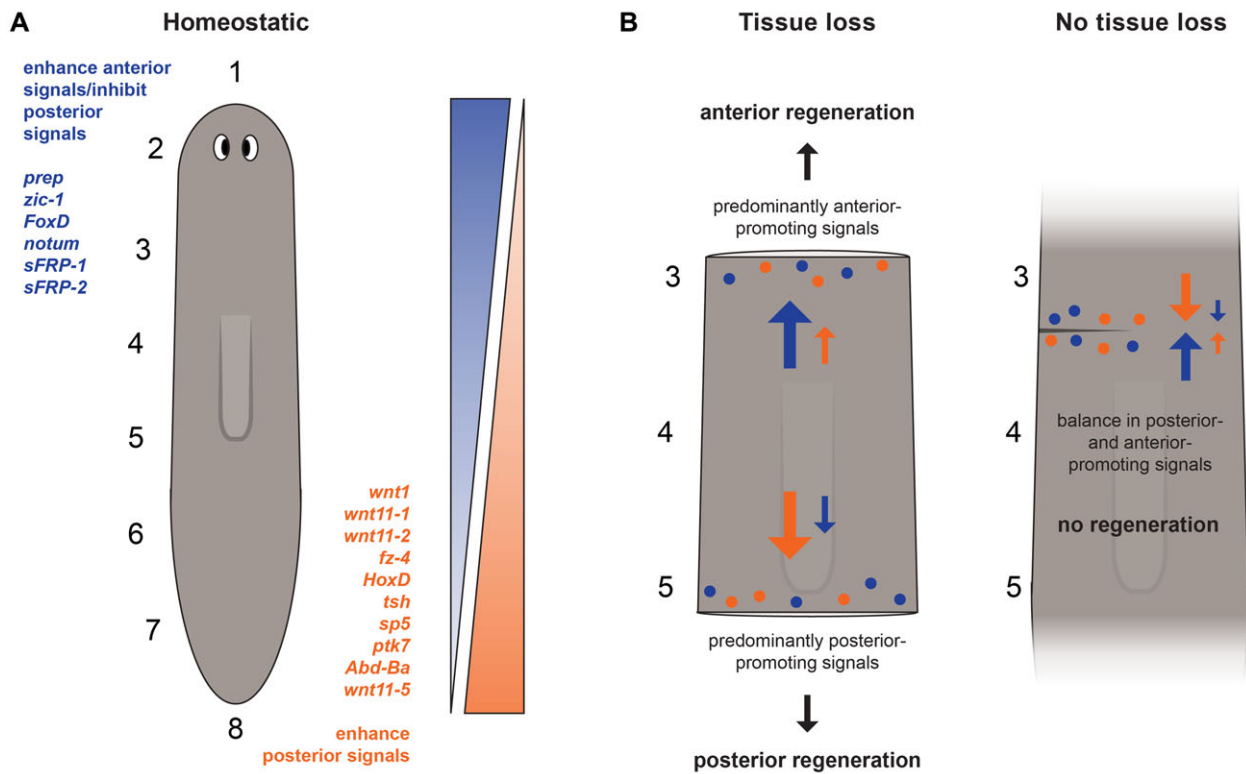
Figure 3. Graded competences along the body axes and their interactions with wound-induced patterning signals may determine the regenerative outcome. (A) Under homeostatic conditions, posteriorizing signals (e.g., Wnt1) are expressed in the tail (orange gradient), while their inhibitors (e.g., Notum) are more highly expressed in the anterior (blue gradient). This creates graded competences along the AP axis, resulting in anterior tissues that are more competent to produce and respond to anterior-promoting signals and less competent to produce and respond to posterior-promoting signals, and vice versa. (B) Anterior- and posterior-promoting patterning genes are wound induced (blue and orange dots) and communicate with surrounding positional information in the existing tissues. Because of the graded competence of cells in this tissue, neighbor-to-neighbor interactions and interactions with wound-induced signals may result in predominantly anterior-promoting signals (blue arrows) at anterior-facing blastemas and posterior-promoting signals (orange arrows) at posterior-facing blastemas of amputated animals. In contrast, anterior-promoting and posterior-promoting signals may be balanced at incisions that do not involve tissue loss, resolving the wound-induced signals and resulting in no regeneration.
