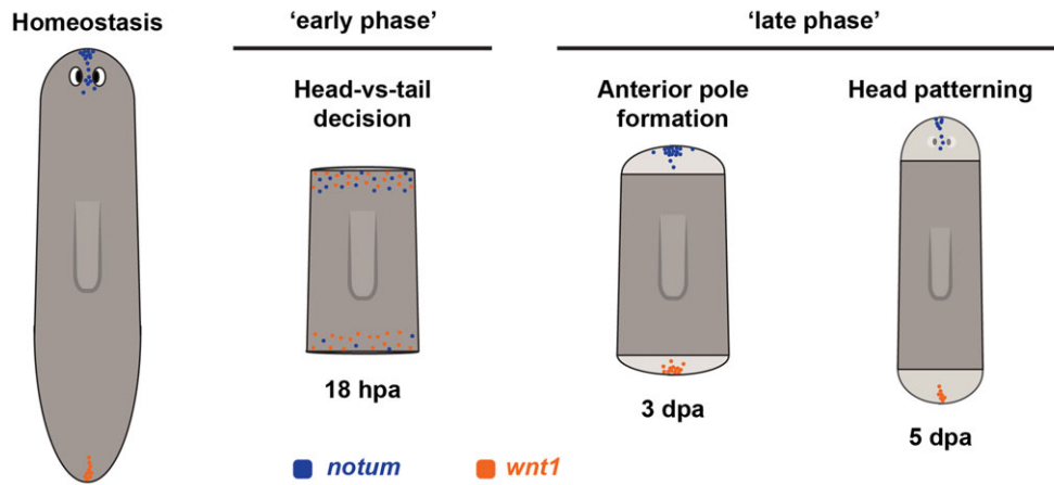
Figure 1. Two phases of wnt1/notum expression and function. In uninjured animals, notum is expressed at the anterior pole and anterior commissure in the brain, while wnt1 is expressed at the posterior pole. During regeneration, both genes are induced at all wounds in a dispersed 'salt and pepper' pattern in the early phase, although notum expression is higher in anterior-facing blastemas. In the late phase, notum and wnt1 expression clusters at the anterior-most and posterior-most tips of the fragment, respectively, the regeneration poles. As regeneration continues, notum and wnt1 expression domains elongate until the homeostatic pattern is restored.
