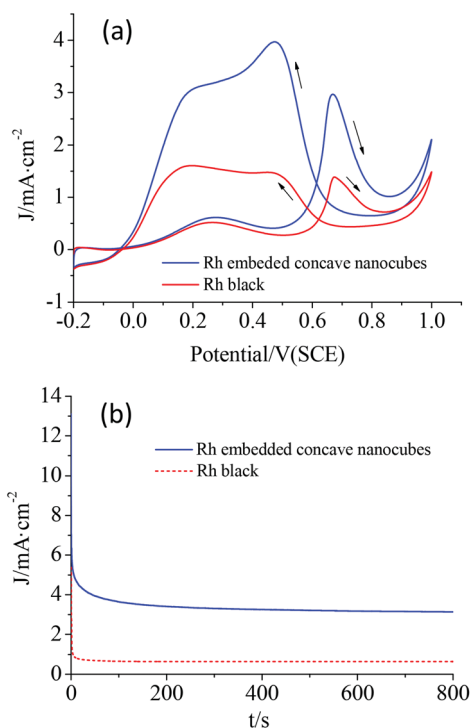
Fig. 6 The CV (a) and CA (b) curves of the mutually embedded Rh concave nanocubes and Rh black in 0.1 M HClO 4 + 0.5 M HCOOH solutions with the cyclic potential between -0.2 and 1.0 V at a sweep rate of 50 mV s -1 .
