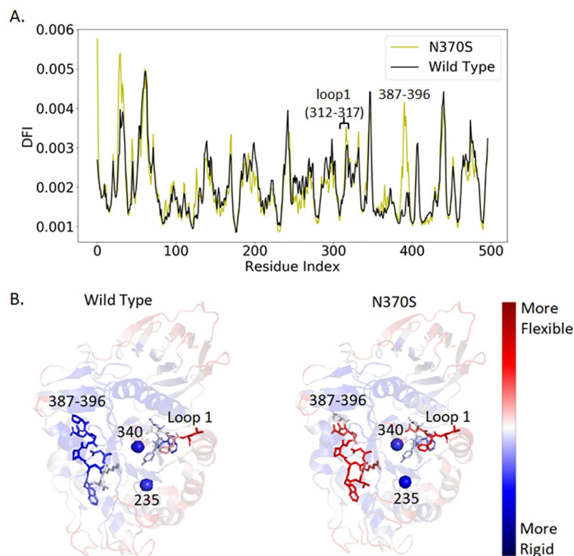
Fig 2. A comparison of DFI profiles of wild-type GCase and N370S mutant protein. (a) The %DFI profile of the mutant protein ( N370S , yellow) is contrasted with that of the wild-type (black). Dissimilarities in the two profiles demonstrate how a single point mutation ( N370S ) can induce changes in the flexibility profile of a different region of the protein. (b) Ribbon diagrams showing DFI as a color-coded spectrum from red-white-blue; red and blue indicate the highest and lowest flexibility, respectively. The regions with the most significant changes in dynamic flexibility are highlighted.
