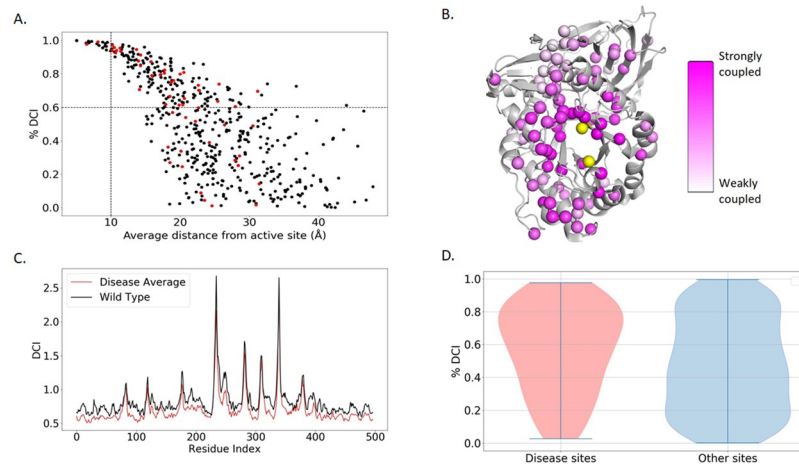
Fig 3. DCI of GCCase sites. (a) Scatter plot of all GCCase residues with dividers at %DCI = 60 and distance = 10 Å. The upper right quadrant contains DARC sites which can affect the active site without direct interaction. Red dots indicate severe DAVs, which have a significantly higher DCI ( P < .001 ) than other sites. (b) A ribbon diagram showing known mutation sites of GCCase (represented as pink-colored dots) and the degree of coupling to the active site delineated by the color gradient, where darker and lighter shades correspond to strongly coupled and weakly coupled, respectively. (c) Average DCI profile of 20 different DAVs compared to the wild-type. In general, we observe a global loss of coupling to the active site. (d) Violin plots showing that DAVs are generally located at sites that have higher DCI with the active site.
