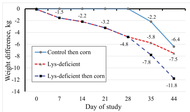
Figure 2. Body weight change relative to control (black horizontal line) when pigs initially 90 kg body weight were fed 1) the control diet for 28 d and then switched to corn-vitamin-trace mineral diet for the final 16 d, 2) fed a lysine-restricted diet for the entire 44 d study, and 3) fed a lysine-restricted diet for the first 28 d of the study followed by a corn-vitamin-trace mineral diet for the final 16 d. The control, lysine-deficient, and corn-vitamin-trace mineral diets contained 0.7%, 0.5%, and 0.18% digestible lysine, respectively. Adapted from Rao et al. (2020b).
