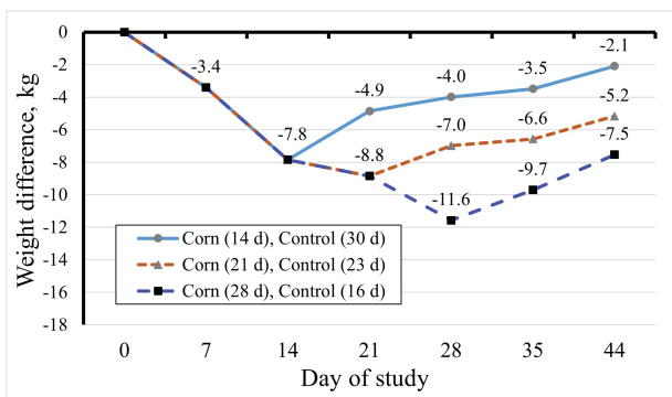
Figure 3. Body weight change relative to control (black horizontal line) when pigs initially 89 kg body weight were fed 1) the corn-vitamin-trace mineral diet for 14 d and then switched to control diet for 30 d, 2) the corn-vitamin-trace mineral diet for 21 d and then switched to control diet for 23 d, and 3) the corn-vitamin-trace mineral diet for 28 d and then switched to control diet for 16 d. The control and corn-vitamin-trace mineral diets contained 0.7% and 0.18% digestible lysine, respectively. Adapted from Rao et al. (2020a).
