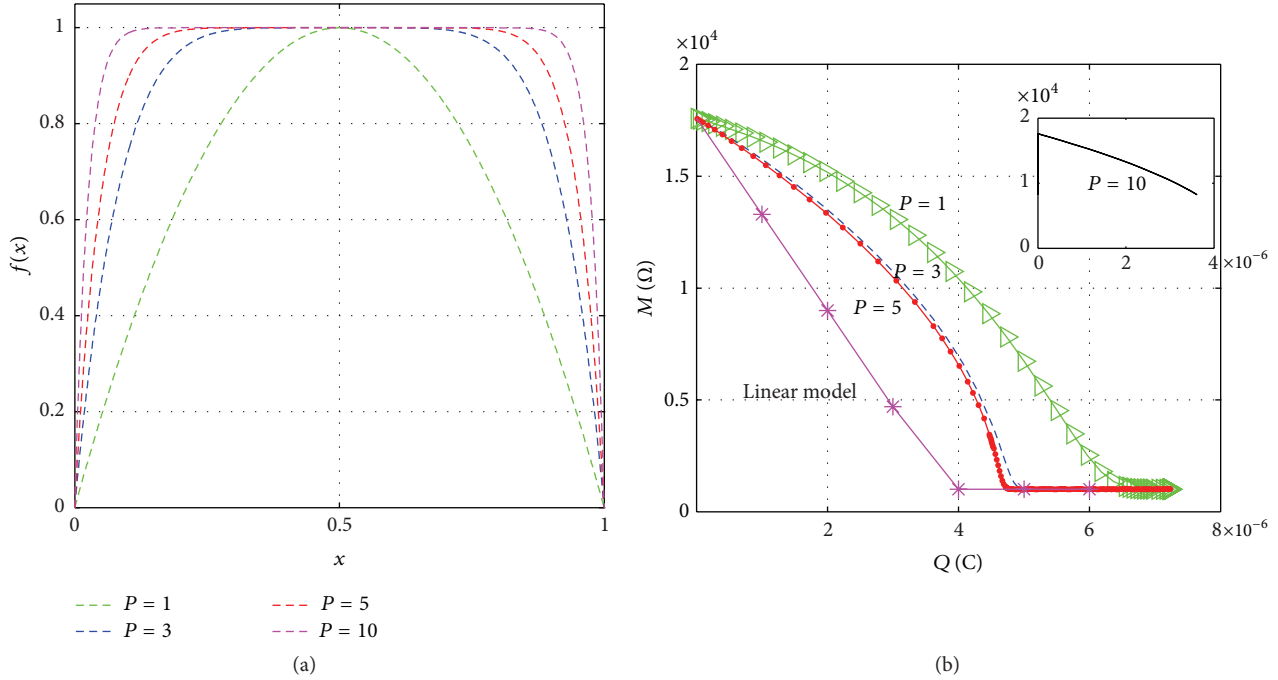
FIGURE 2: The influence of different values of the integer P on the memristor. (a) Joglekar window function for P = 1, P = 3, P = 5, and P = 10 . (b) Relationship between memristance versus charge for the nonlinear memristor model. As the integer P increases, the graphs tend to linearity.
