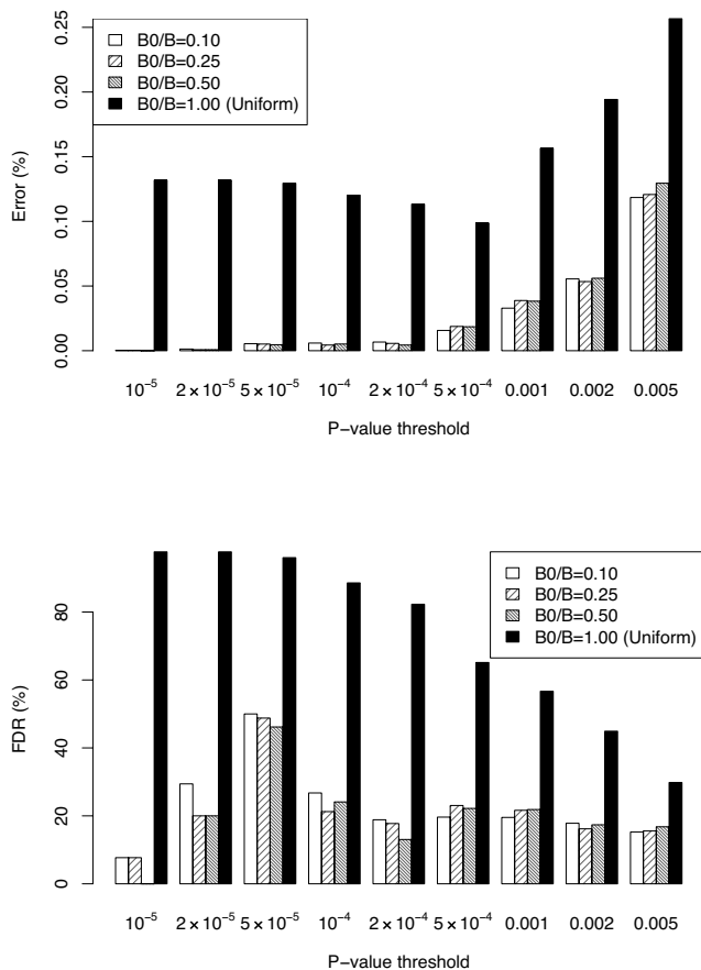
Figure 3 Sample figure title. Error (defined as (FN+FP)/(P+N) ) and false discovery rate of the uniform ( B_0/B_0 = 1 ) and differential allocation algorithms using the public Parkinson Disease genome-wide association study dataset.
