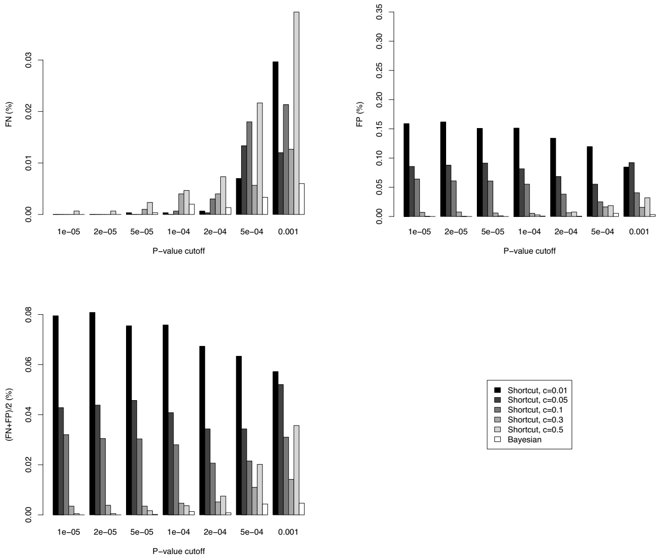
Figure 4 Sample figure title. FN, FP, and Average Error (defined as (FN+FP)/2 ) of the shortcut and our differential allocation algorithm (bayesian) in our simulation study. The value c in the legend is the level of confidence interval used in the shortcut method; see text for more details.
