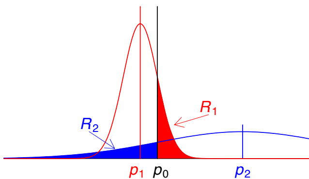
Figure 1 Sample figure title. Illustration of the risks associated with two different p-values. The red density is the posterior distribution of p-value p_1 . The blue density is the posterior distribution of p-value p_2 . The decision threshold for assessing significance is denoted as p_0 . The risk R_1 (associated with p-value p_1 ) is the red area on the right of the decision threshold p_0 . The risk R_2 (associated with p-value p_2 ) is the blue area on the left of the decision threshold p_0 .
