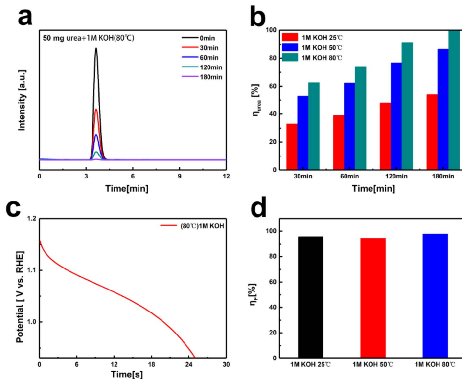
Fig. 5 (a) HPLC of urea decomposition on \text{Ni}(\text{OH})_2 electrode in 1 M KOH concentration at 80 °C with the addition of 1 \text{ g L}^{-1} urea over 0–180 minutes. (b) The urea conversion rates at 25 °C, 50 °C, and 80 °C. (c) Discharge curve of \text{Ni}(\text{OH})_2 electrode after 180 minutes of urea decomposition in 1 M KOH concentration at 80 °C at 100 mA. (d) The corresponding faradaic efficiencies of urea decomposition at \text{Ni}(\text{OH})_2 electrodes with 25 °C, 50 °C, and 80 °C.
