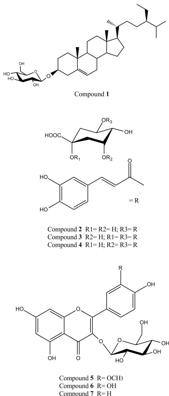
Figure 1. Structures of the isolated compounds from the aerial parts of D. glabrum .
