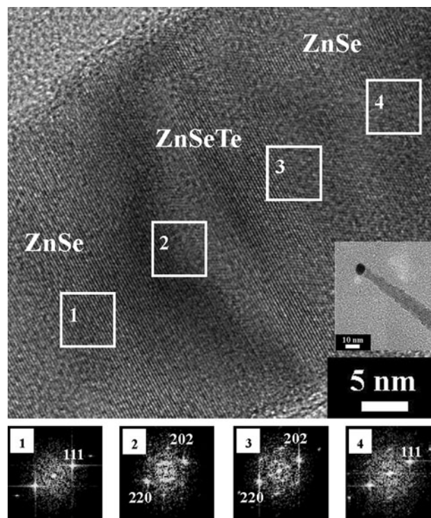
Fig. 3 HRTEM image of one randomly selected ZnSe/ZnSeTe superlattice nanotip with L_w = 20 nm. Insets at the bottom show FFT patterns measured from four different points in this particular superlattice nanotip and low-magnification bright-field TEM image
