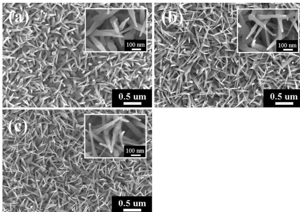
Fig. 2 Top-view FESEM images of the ZnSe/ZnSeTe superlattice nanotips with L_w = a 16 nm, b 20 nm, and c 24 nm, respectively
