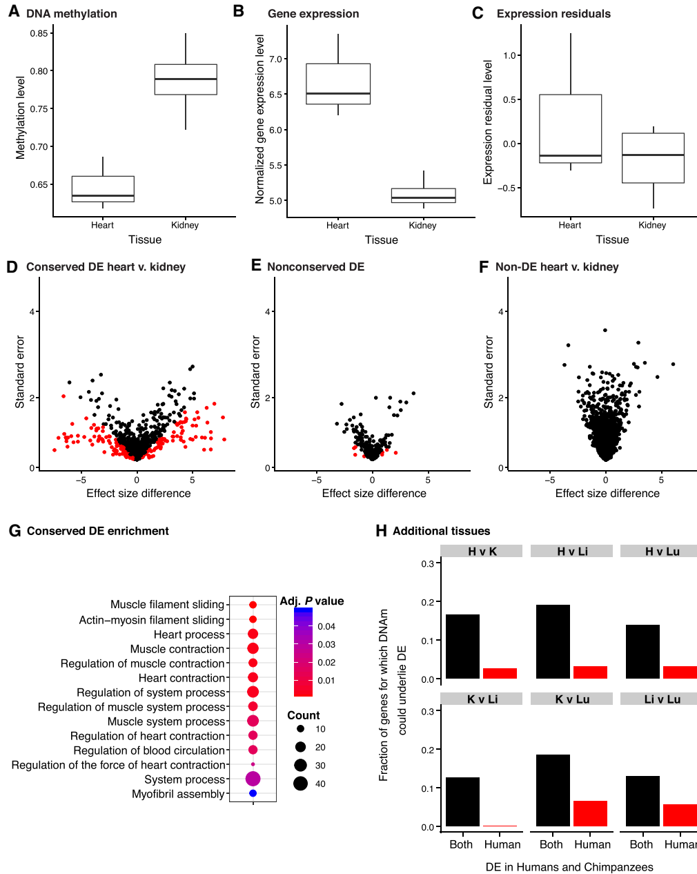
Figure 4. Inter-tissue DNA methylation and gene expression levels (FDR=0.05 and FSR=0.05). (A–C) A representative example of the PRKACA gene in which the variation of methylation levels (A) may explain the differences in gene expression levels (B) between human heart and kidney. (C) The residuals of normalized gene expression levels after regressing out methylation levels. (D–G) Next, we compared the tissue effect sizes before and after controlling for DNA methylation levels in inter-tissue DE and non-DE genes, separately. Genes in red are significant at S -value < 0.05 . Effect size differences in conserved DE genes in human heart relative to human kidney (D), nonconserved DE genes in human heart relative to human kidney (E), and non-DE genes in human heart and human kidney (F). (G) The conserved DE genes are enriched for heart-related function. (H) Variation in DNA methylation is more likely to explain variation in conserved DE genes than nonconserved DE genes (DE in the human tissues listed, but not in the same tissues in chimpanzees).
