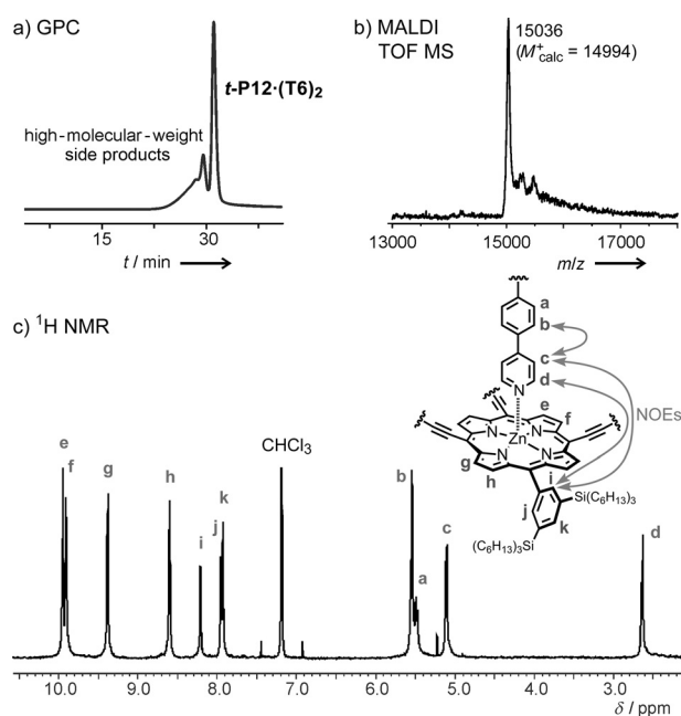
Figure 2. Characterization of t-P12·(T6) 2 : a) GPC chromatogram (529 nm) of the crude reaction mixture. b) MALDI-TOF spectrum. c) Partial 1 H NMR spectrum (400 MHz, \text{CDCl}_3 ) showing selected NOEs.
