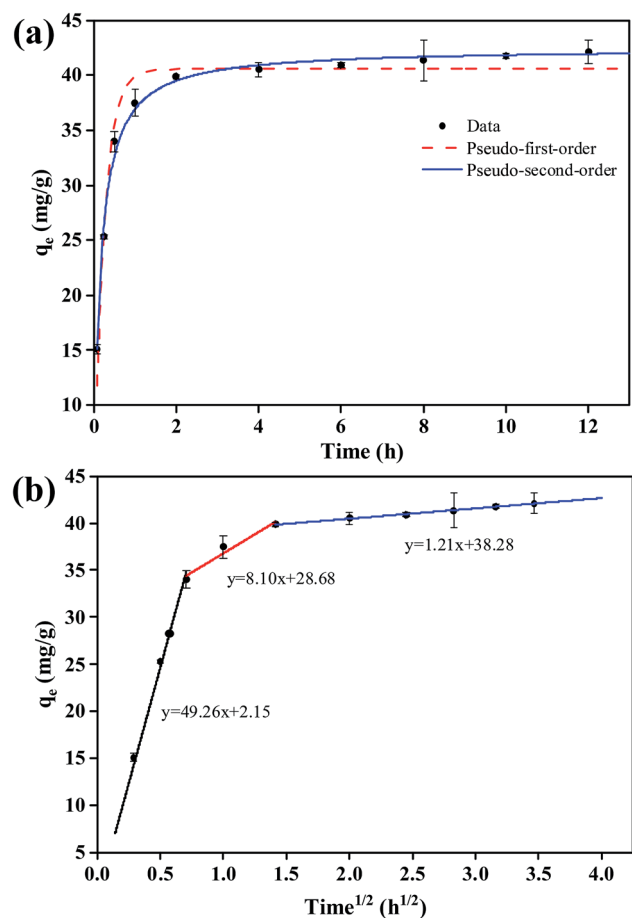
Fig. 5 Kinetics of phosphate adsorption on FCB/MAC: (a) experimental data and fitting for pseudo-first-order and pseudo-second-order models and (b) intraparticle diffusion model. Adsorption conditions: initial phosphate concentration, 50 mg L -1 ; solution pH, 3.0; temperature, 25 °C; FCB/MAC dosage, 0.25 g; working volume, 250 mL; contact time, 12 h.
